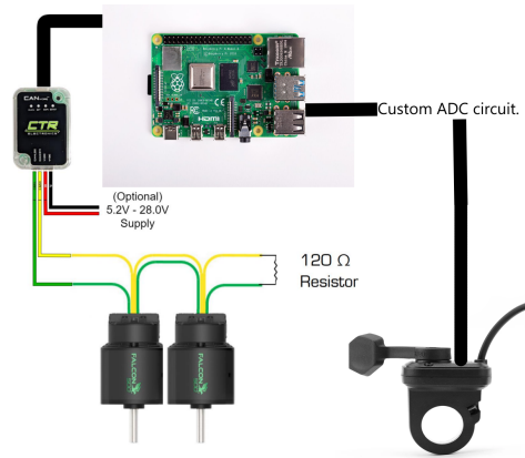
Figure 10: Electric Drivetrain Architecture.
