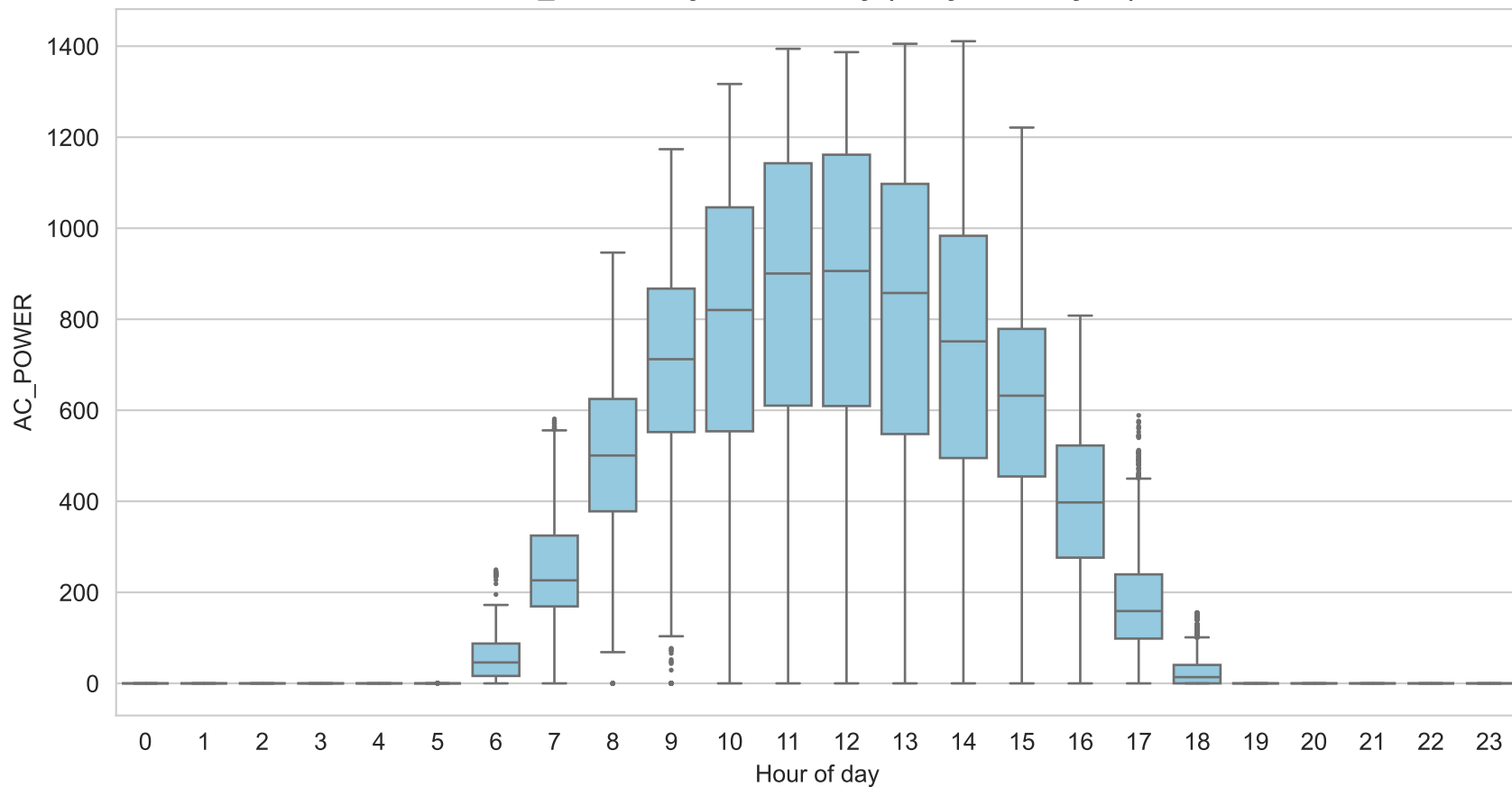
AC_POWER by Hour of Day (Daily Solar Cycle)
