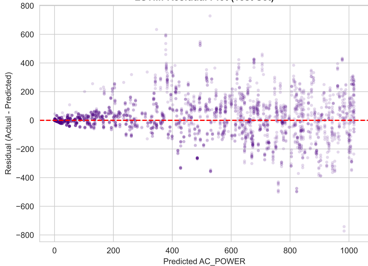
LSTM: Residual Plot (Test Set)
