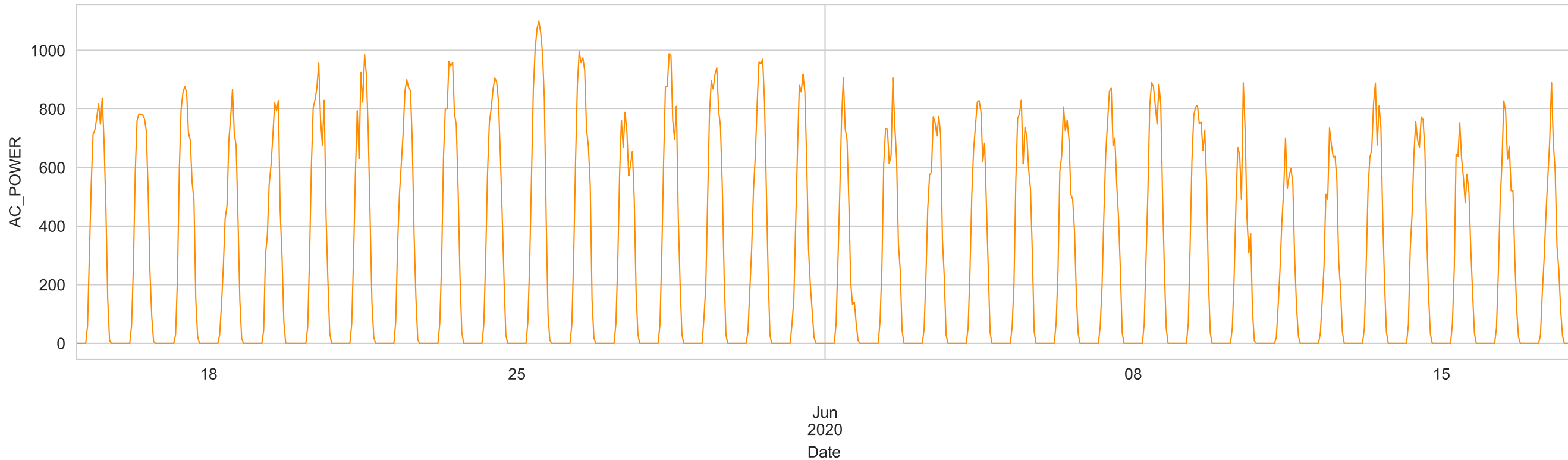
Fleet-Average AC_POWER Over Time (hourly mean)
