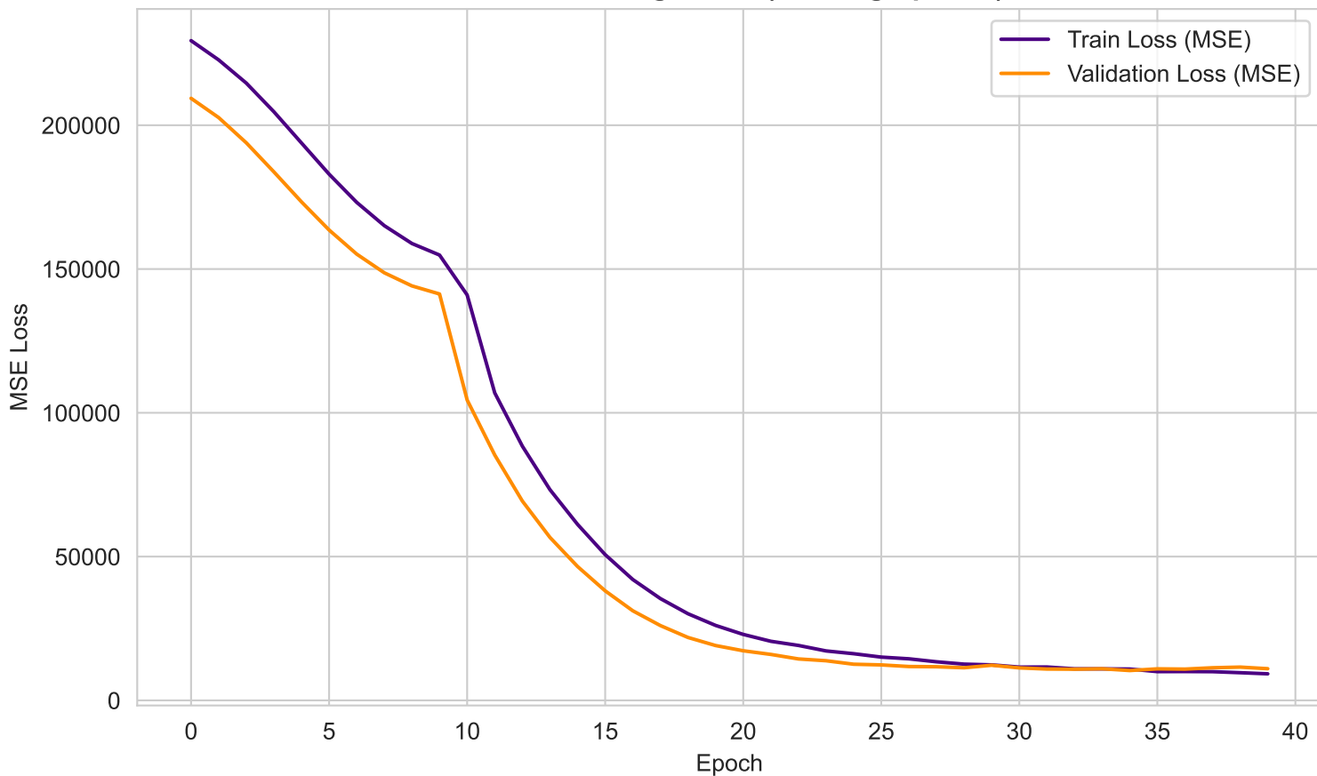
LSTM: Learning Curve (Training Epochs)
