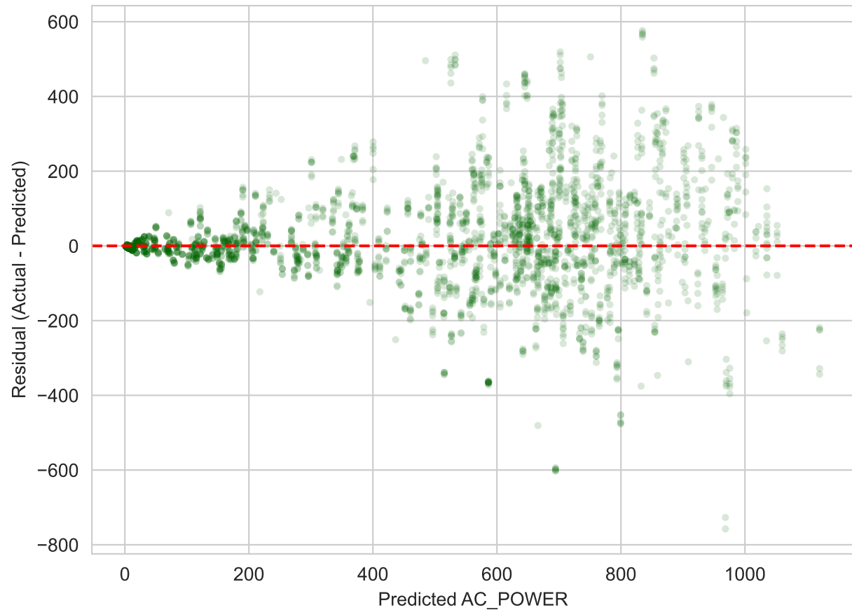
LightGBM: Residual Plot (Test Set)
