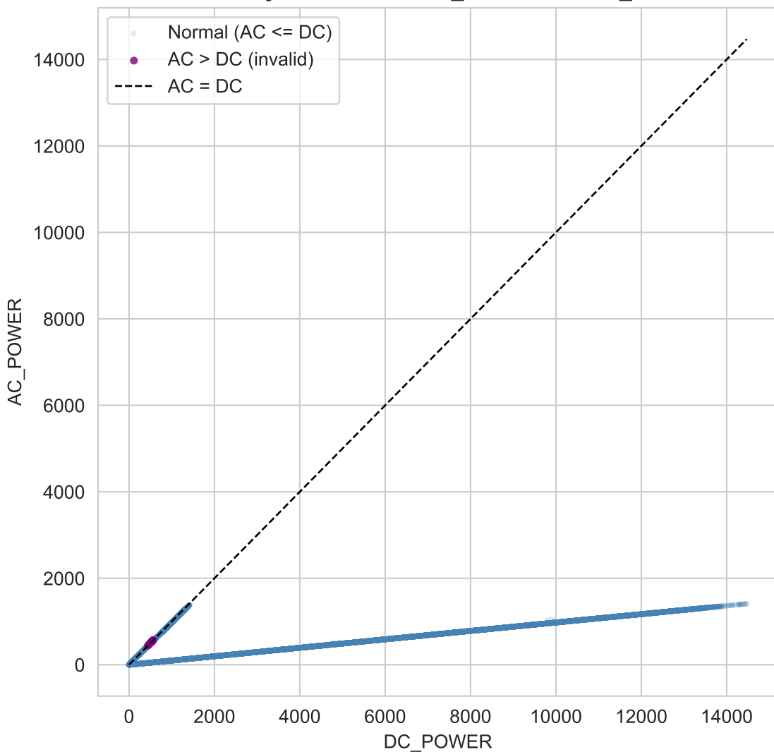
Invalid Physical Values: AC_POWER vs DC_POWER
