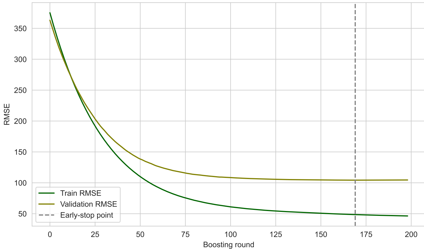
LightGBM: Learning Curve (Boosting Rounds)
