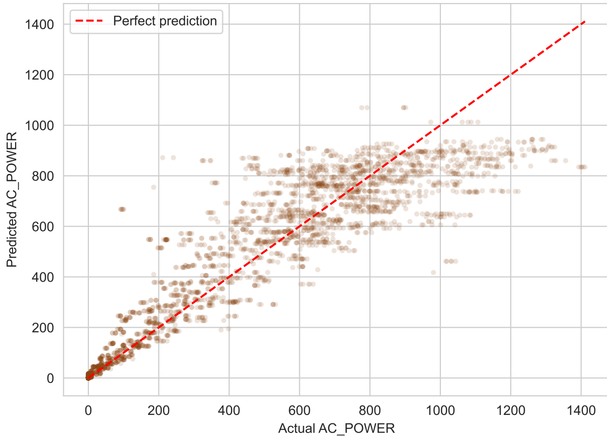
Random Forest: Actual vs Predicted (Test Set)
