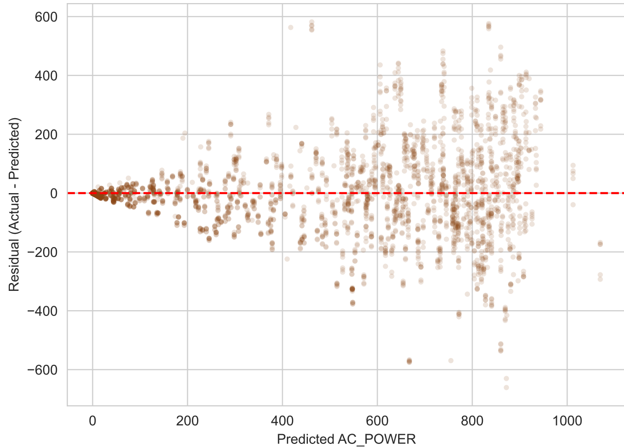
Random Forest: Residual Plot (Test Set)
