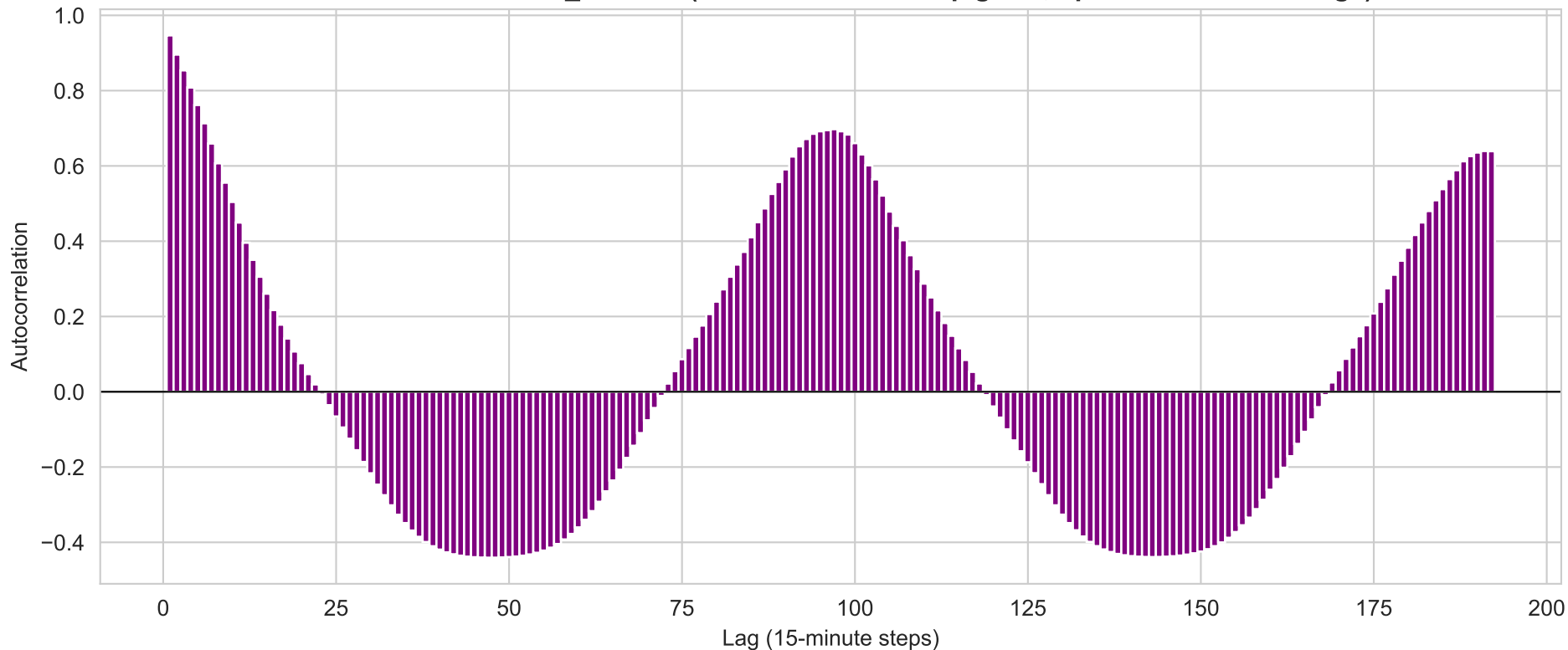
Autocorrelation of AC_POWER (inverter LIT2YUhhzqhg5Sw, up to 48h of 15-min lags)
