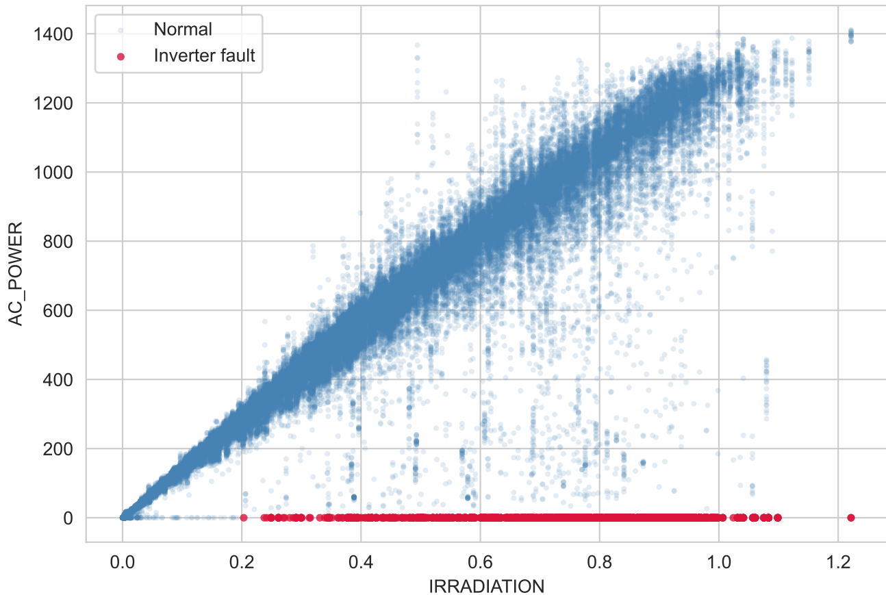
Fault Isolation: IRRADIATION vs AC_POWER
