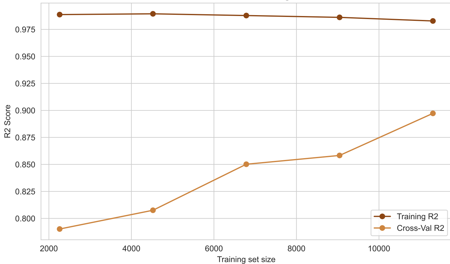
Random Forest: Learning Curve
