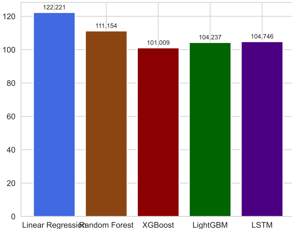
Test RMSE Comparison
