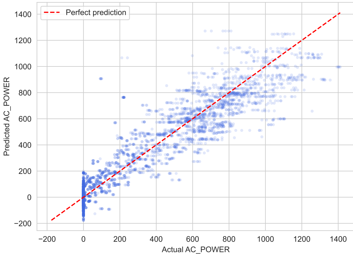
Linear Regression: Actual vs Predicted (Test Set)
