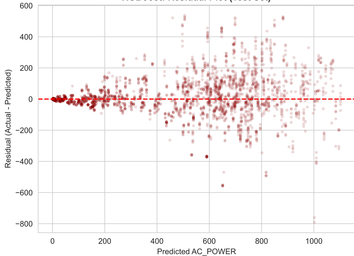
XGBoost: Residual Plot (Test Set)
