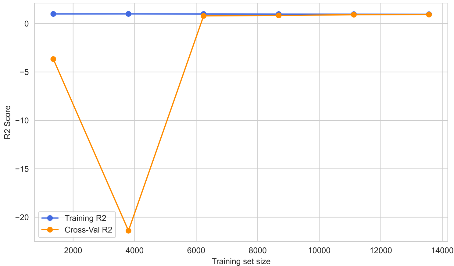
Linear Regression: Learning Curve
