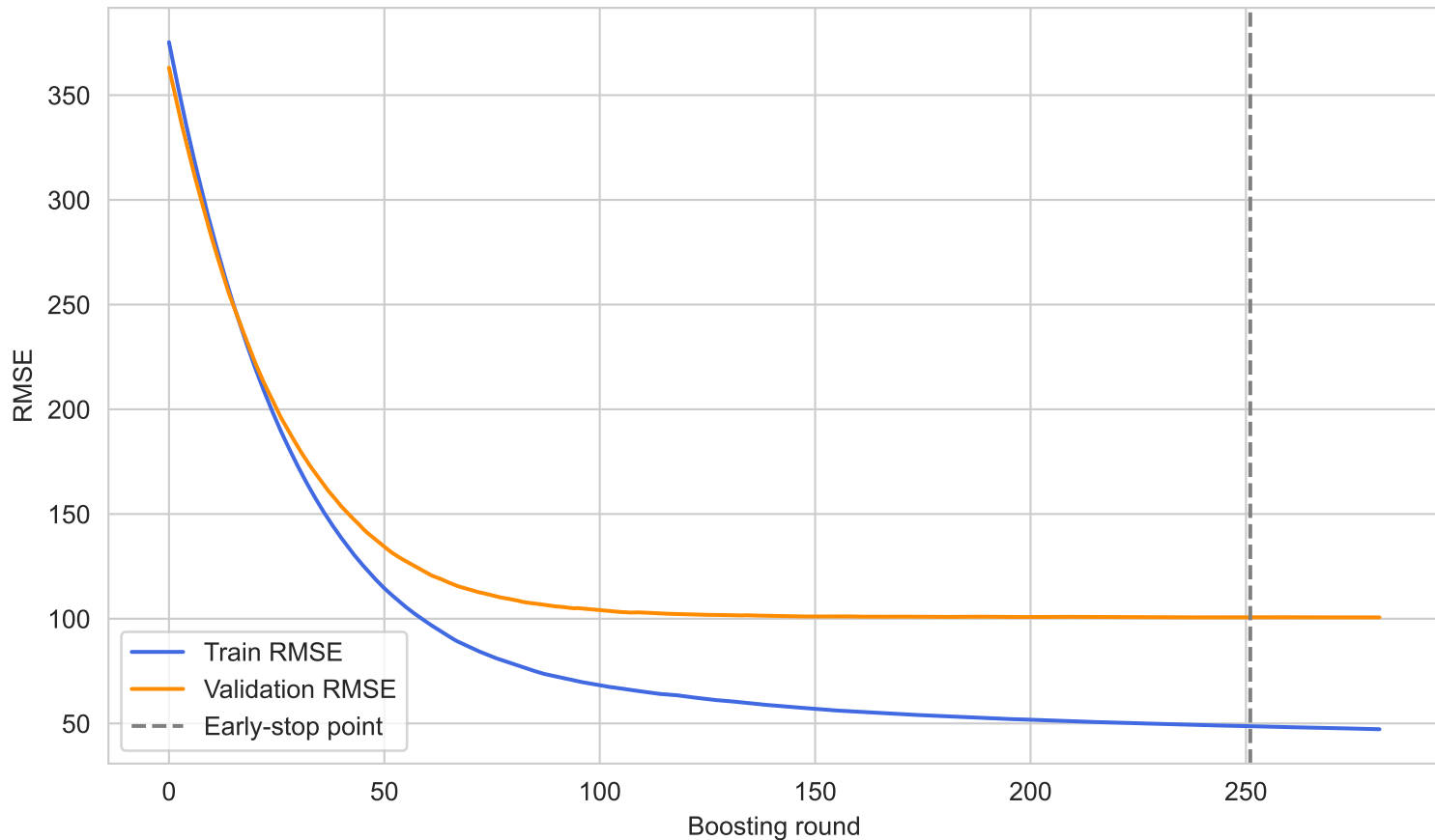
XGBoost: Learning Curve (Boosting Rounds)
