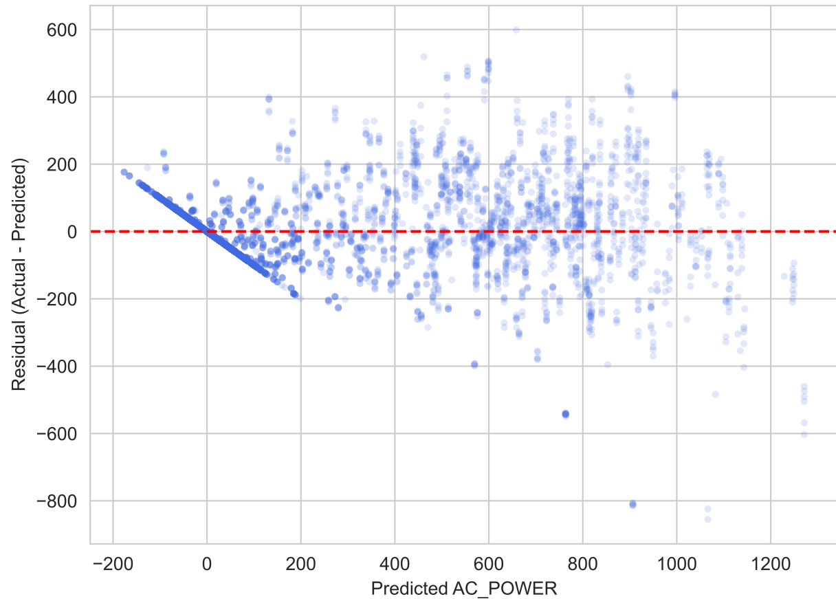
Linear Regression: Residual Plot (Test Set)
