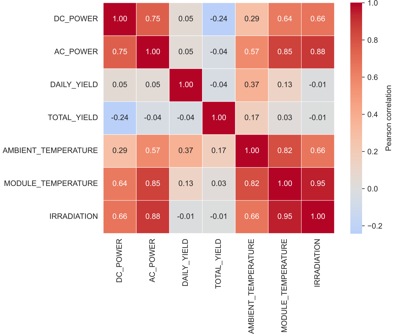
Correlation Heatmap — Sequence Feature Columns
