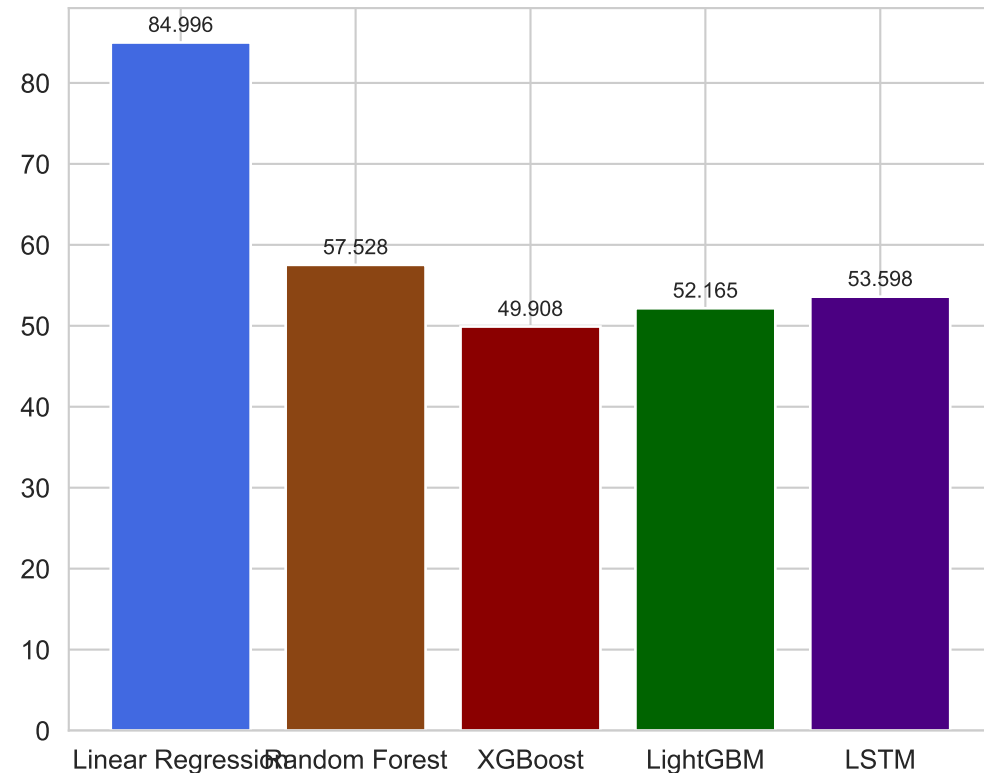
Test MAE Comparison
