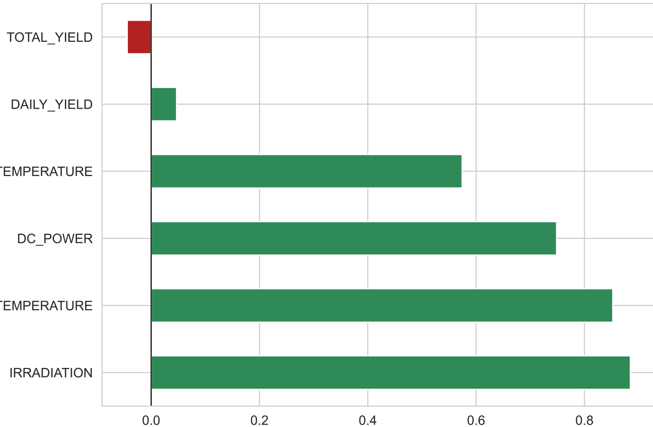
Feature Correlation with AC_POWER
