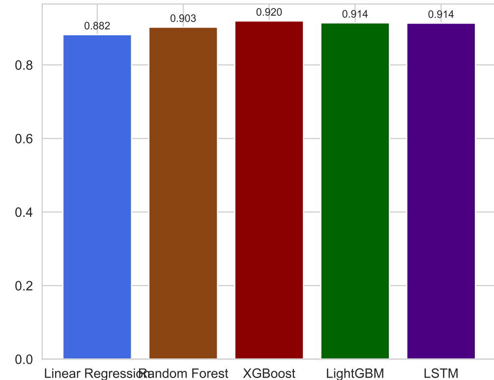
Test R2 Comparison
