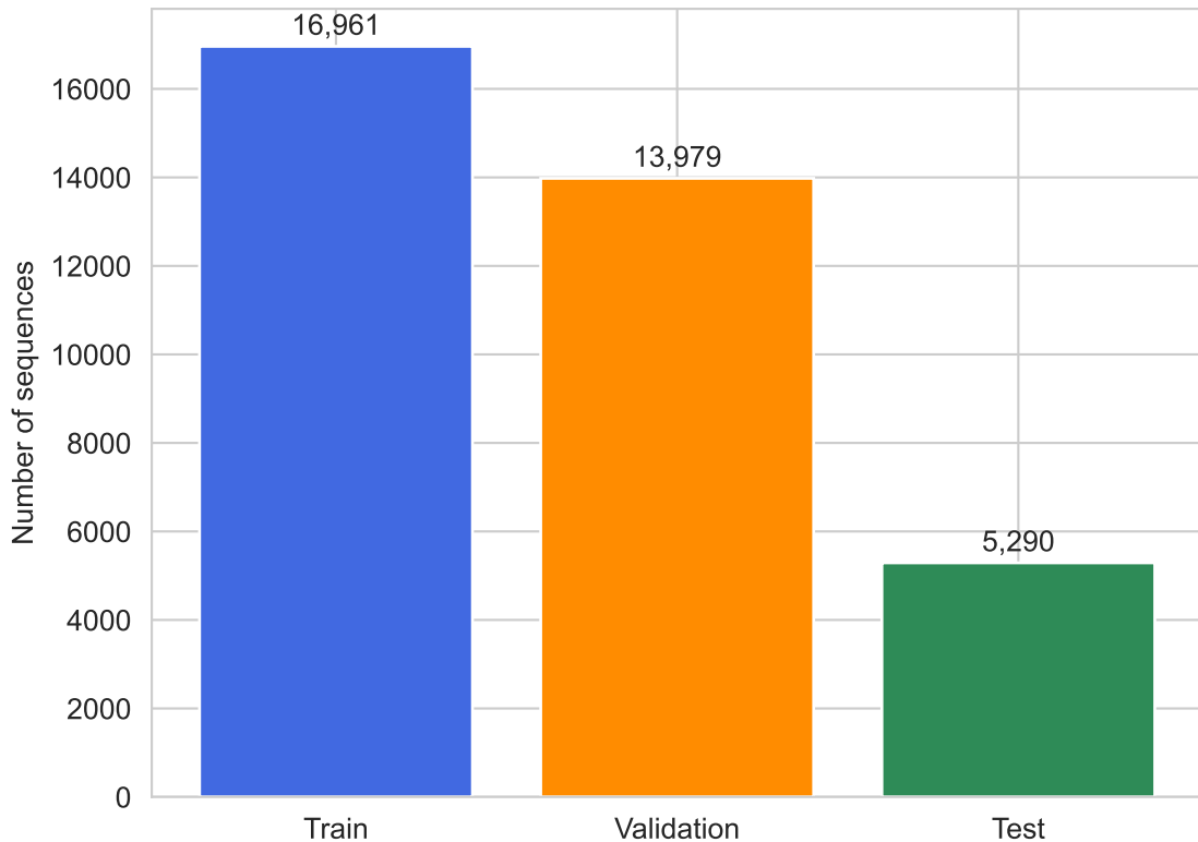
Sequence Count by Split (Chronologically-Ordered Eligible Segments)
