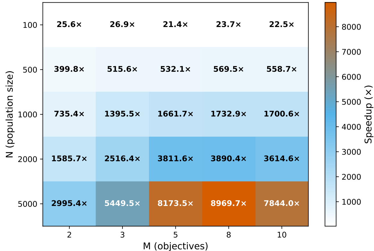
Figure 3: GPU-NDS Speedup over CPU-DCNS
