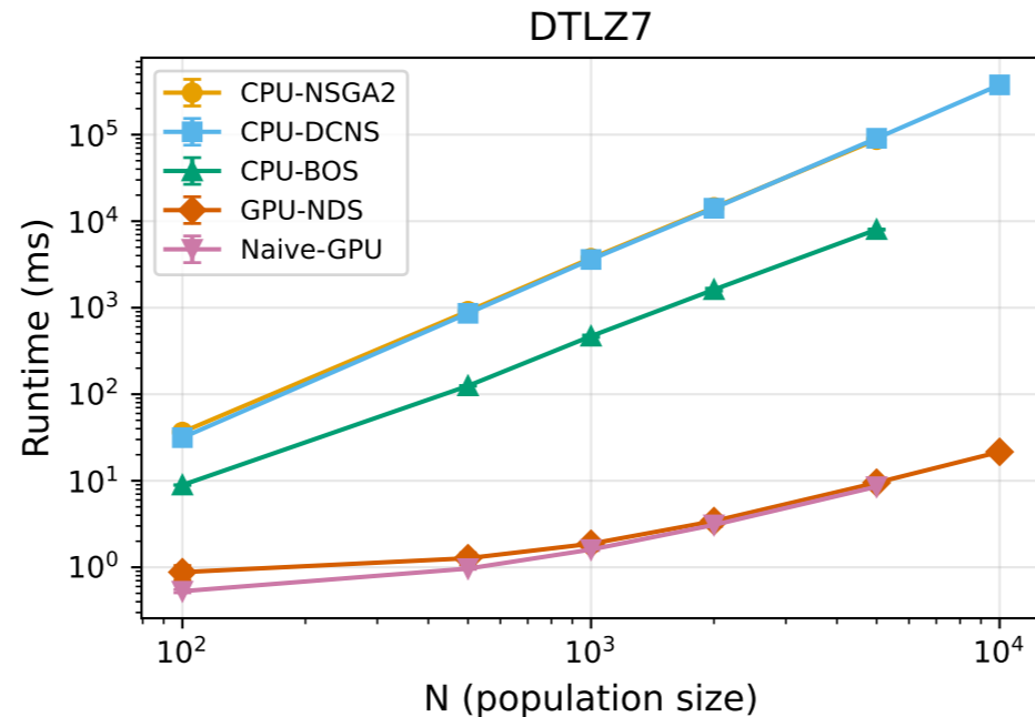
Figure 1: Runtime vs Population Size N
