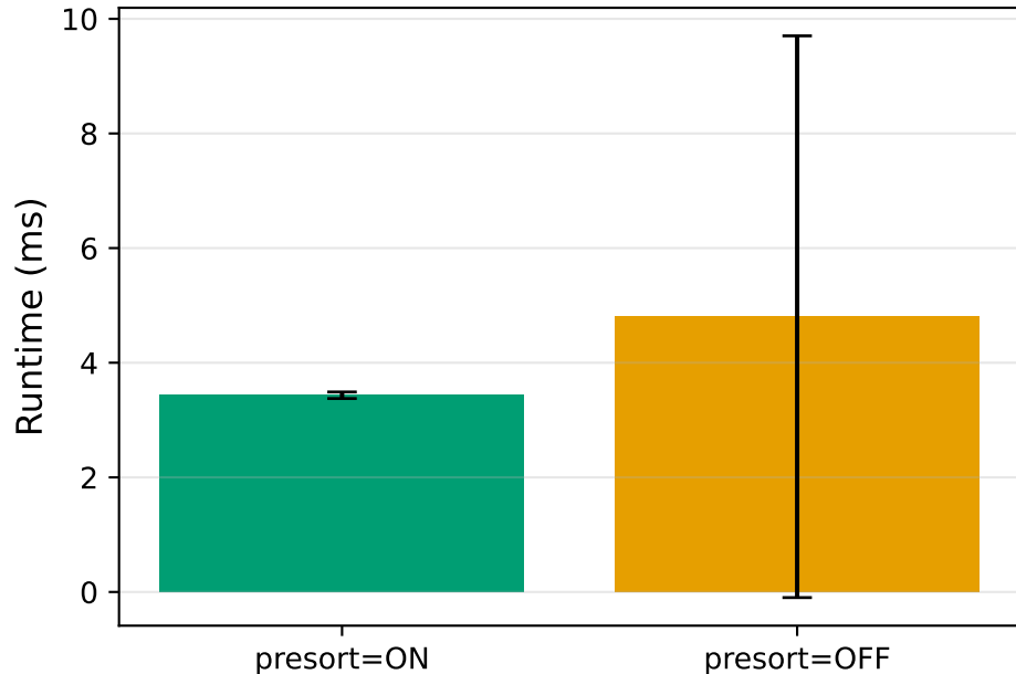
Sum-of-Objectives Presort
