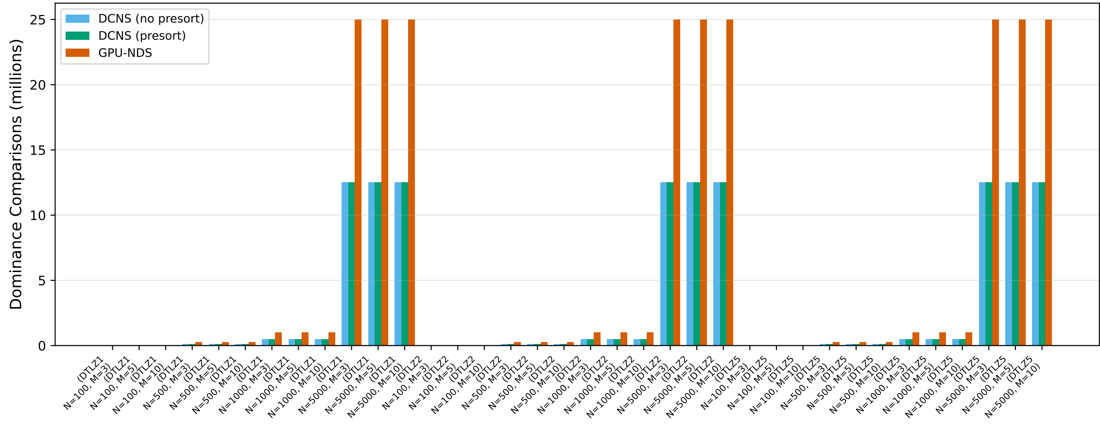
Figure 4: Dominance Comparison Count
