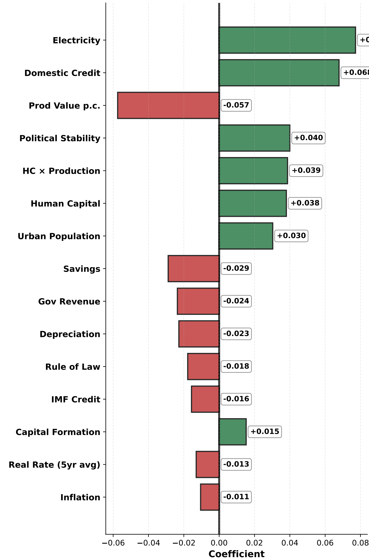
Ridge Train R 2 =0.783 Test R 2 =0.847 | 24 features
