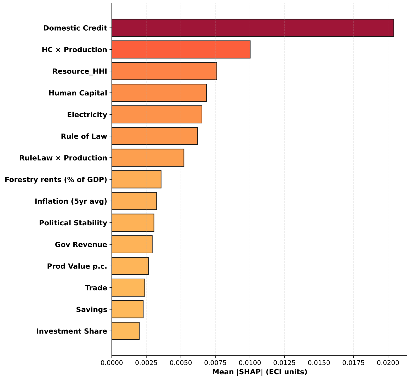
SHAP — Random Forest (test set)
