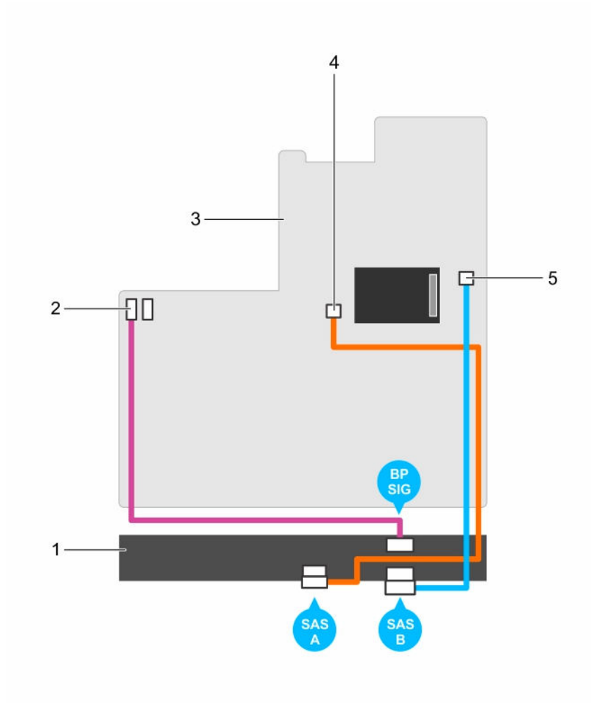
Figure 63. Cabling diagram—2.5 inch (x8) SAS/SATA backplane (option 2)
