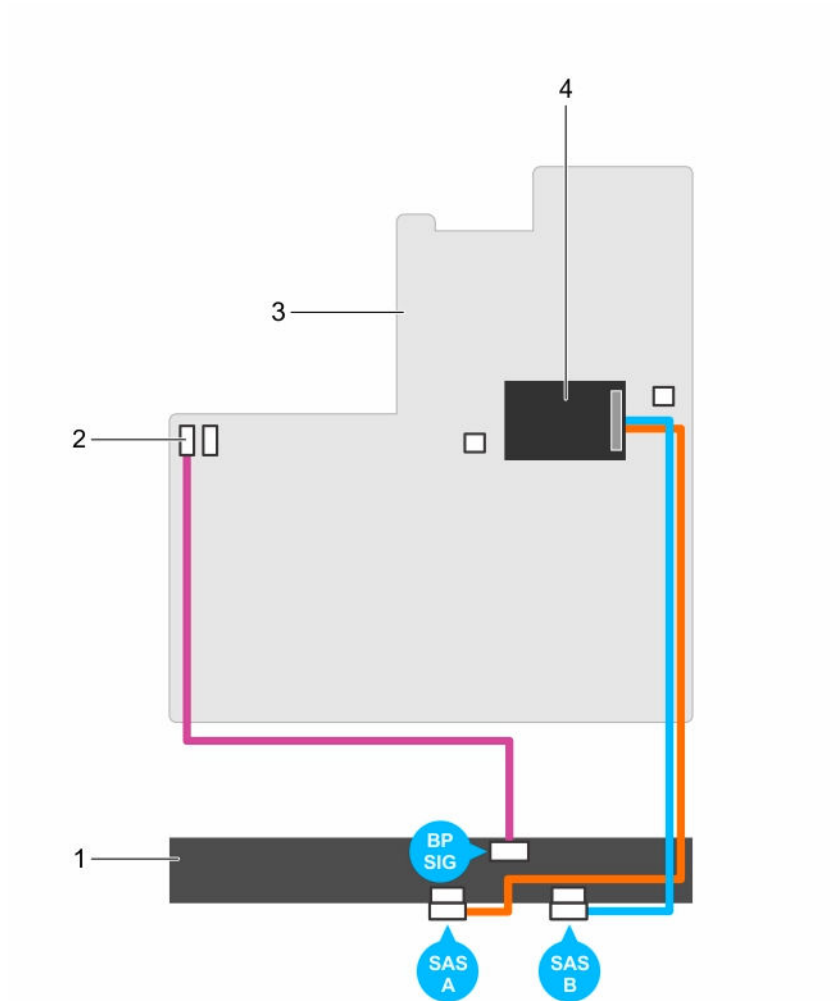
Figure 65. Cabling diagram—3.5 inch (x8) SAS/SATA backplane—(option 1)
