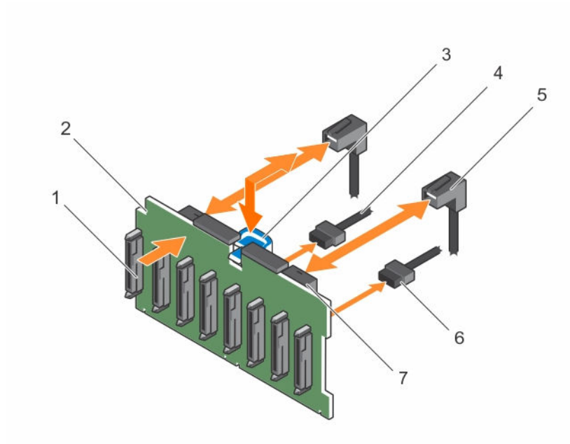
Figure 61. Removing and installing the 2.5 inch (x8) SAS/SATA backplane
