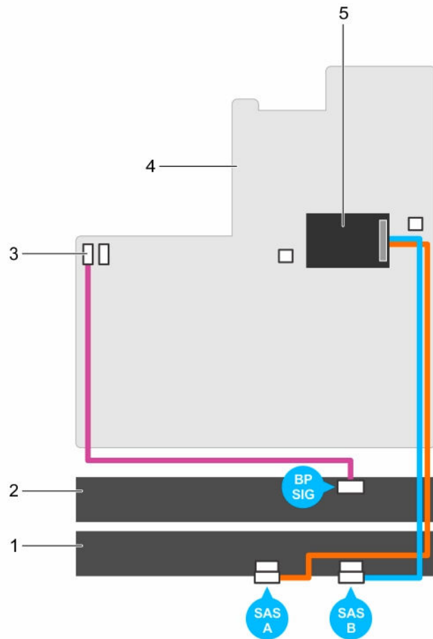
Figure 60. Cabling diagram—2.5 inch (x16) SAS/SATA backplane
