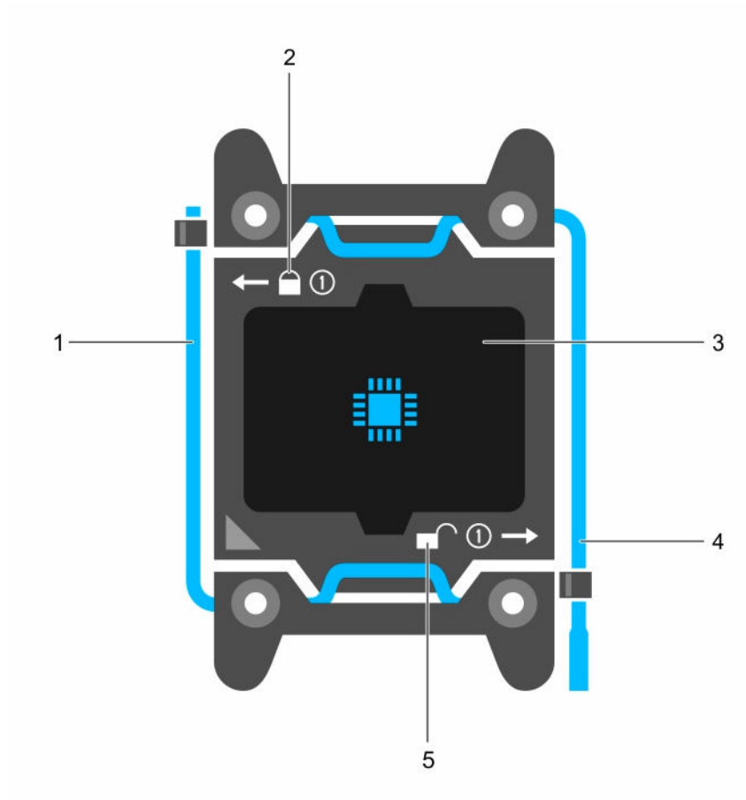
Figure 22. Processor shield
