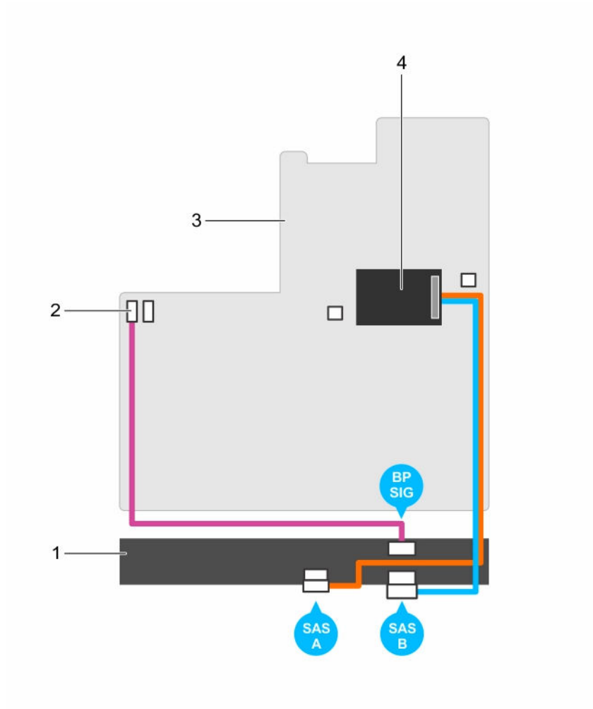
Figure 62. Cabling diagram—2.5 inch (x8) SAS/SATA backplane (option 1)
