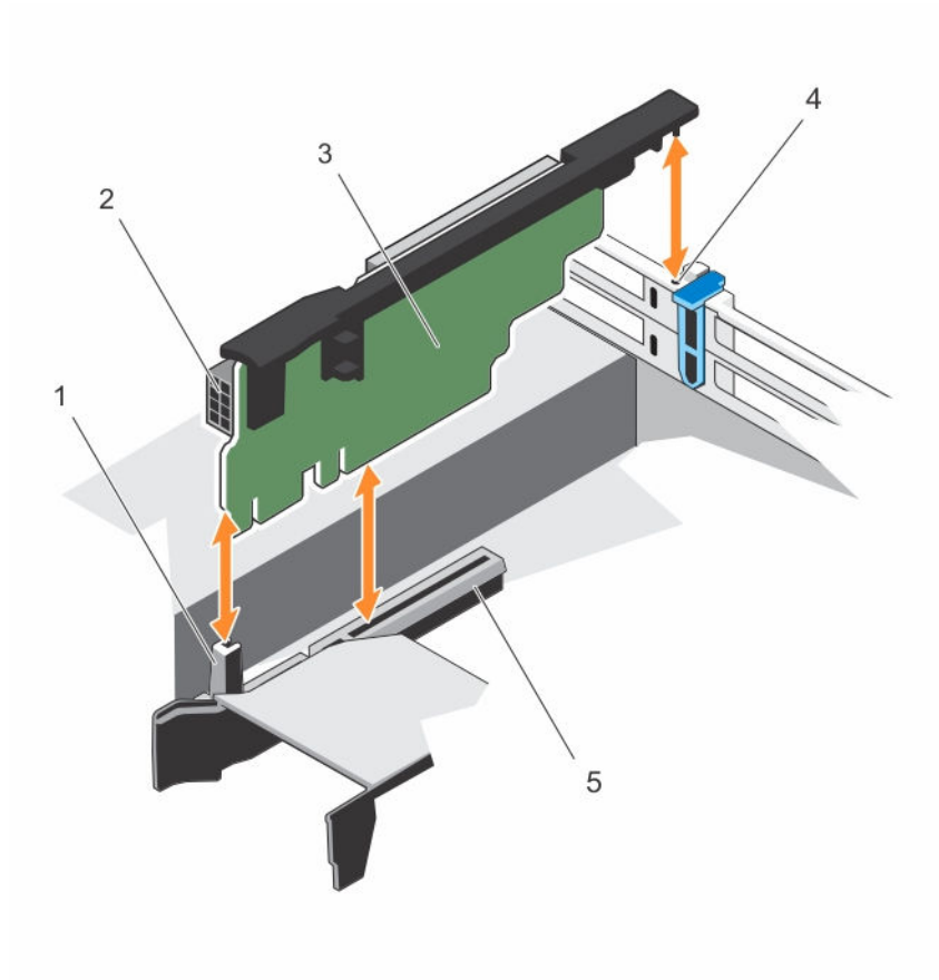
Figure 36. Removing and installing the expansion card riser 3
