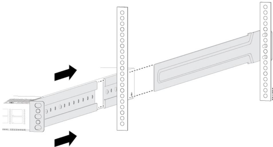
Figure 5: Installing the Switch
