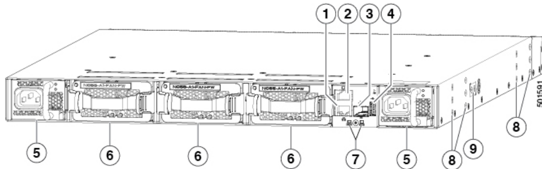
Figure 2: Power Supply Side View of the Cisco N9336C-FX2 Switch
