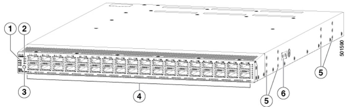
Figure 1: Port Side View of the Cisco N9336C-FX2 Switch
