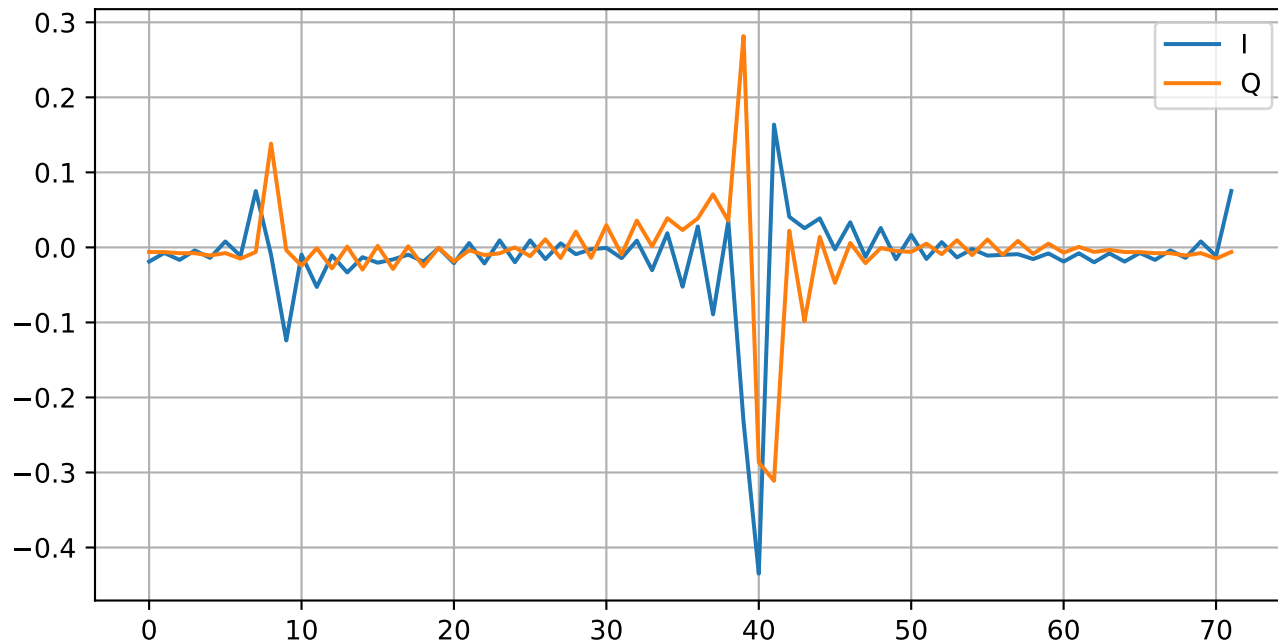
[UFONE] [CLEAN] OFDM (31)
