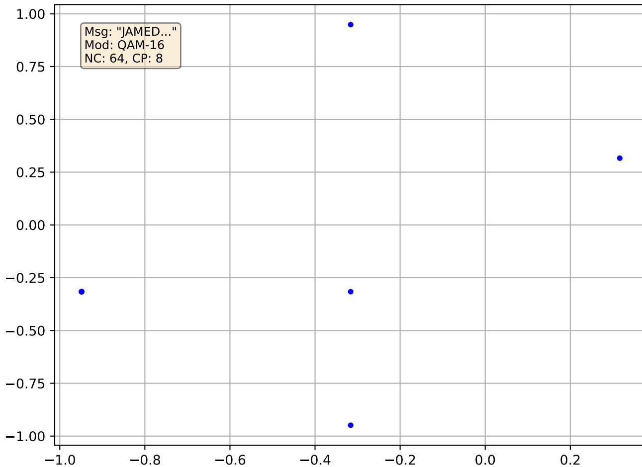
[UFONE] [CLEAN] Constellation (15)
