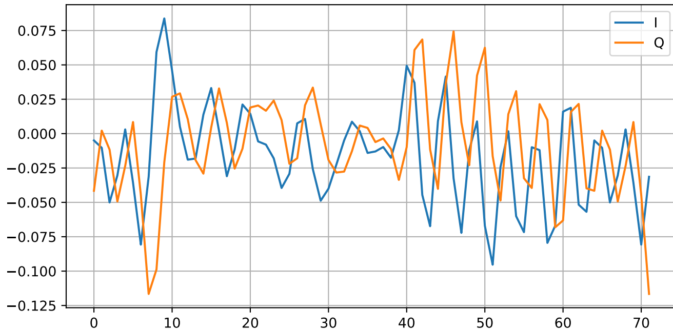
[UFONE] [CLEAN] OFDM (21)
