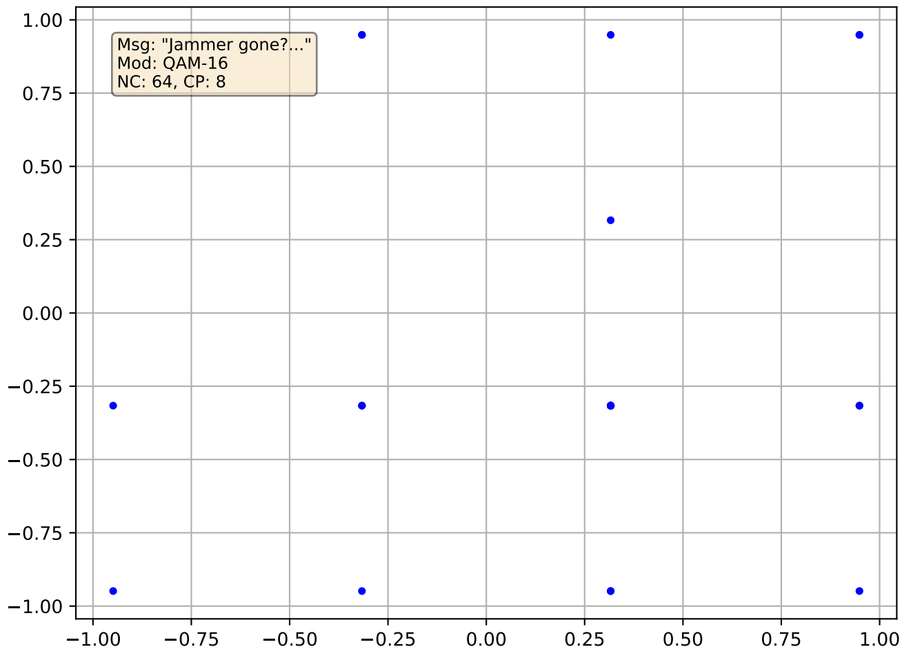
[UFONE] [CLEAN] Constellation (34)
