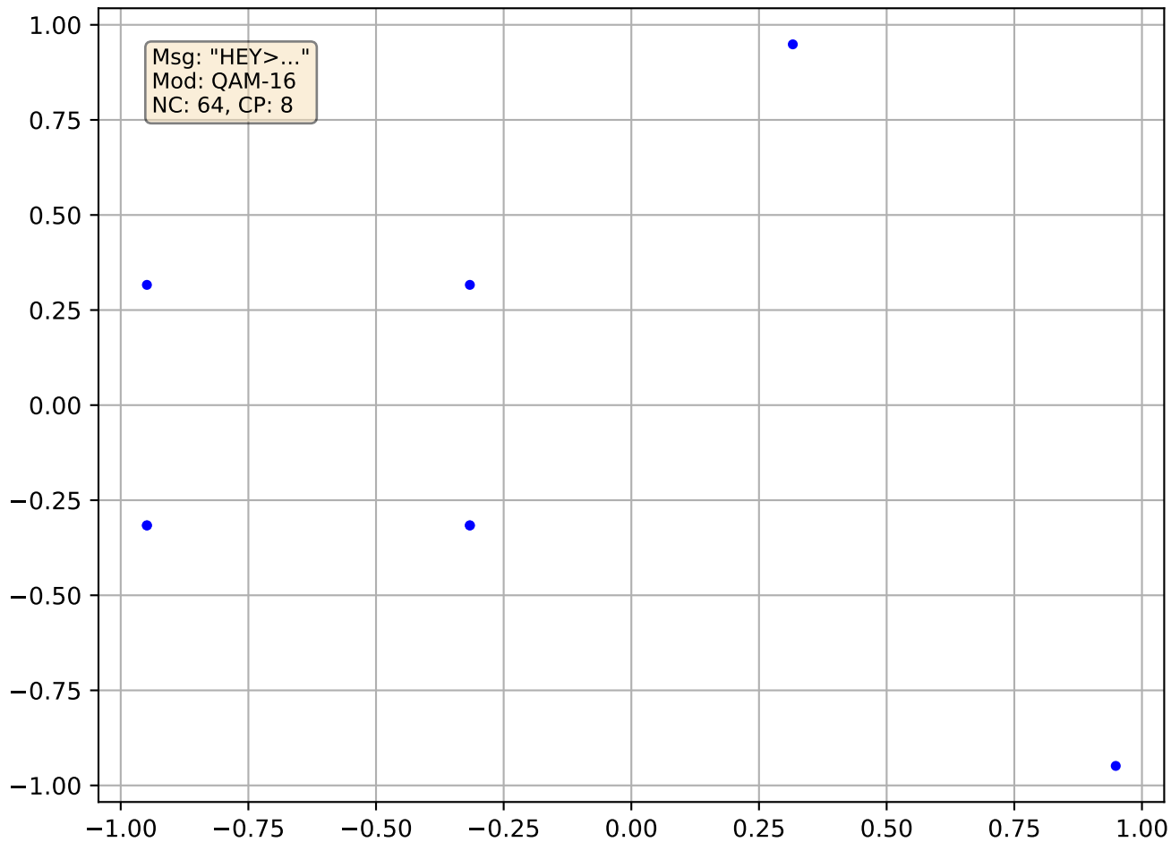
[UFONE] [CLEAN] Constellation (14)
