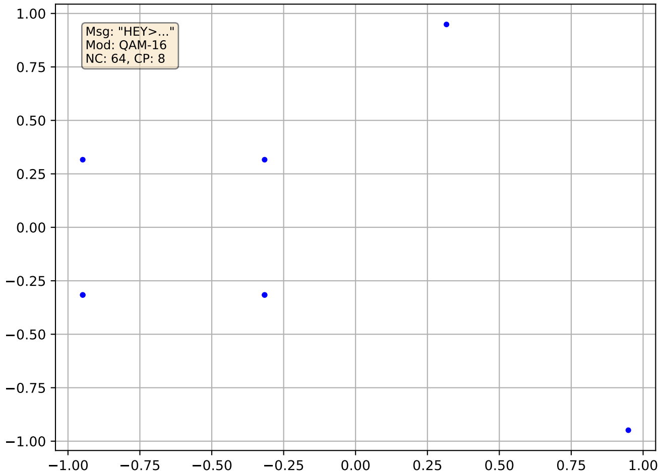
[UFONE] [CLEAN] Constellation (9)
