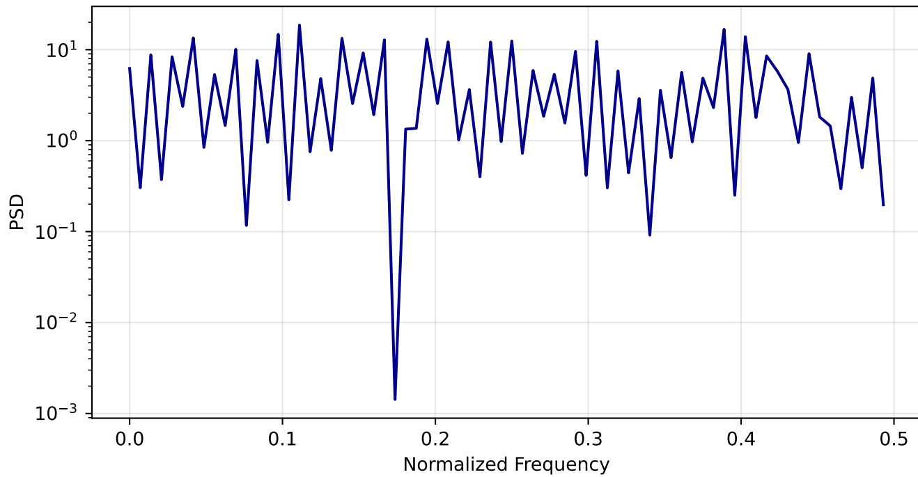
[UFONE] [JAMMED] PSD (11)
