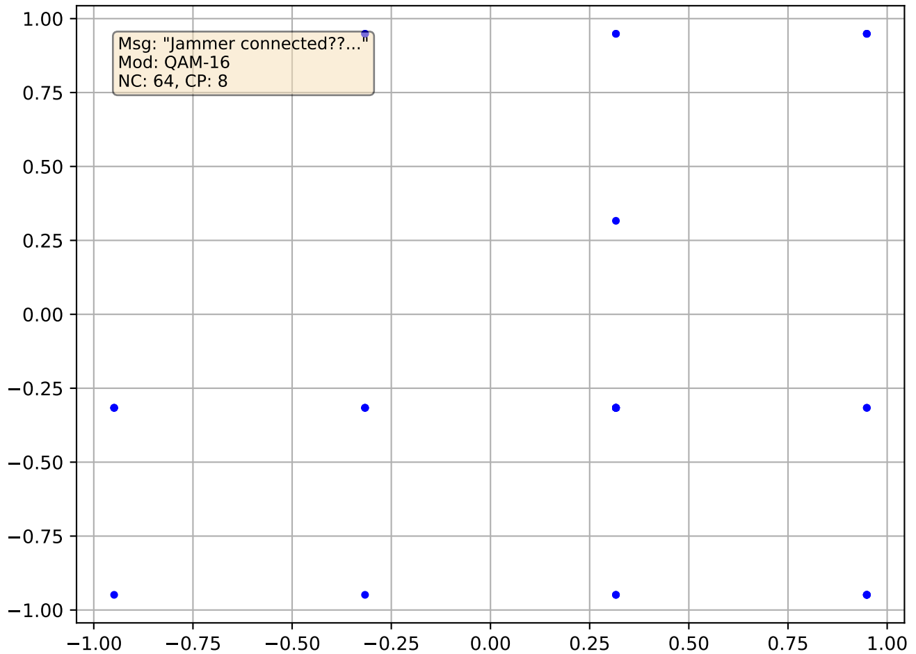
[UFONE] [CLEAN] Constellation (6)
