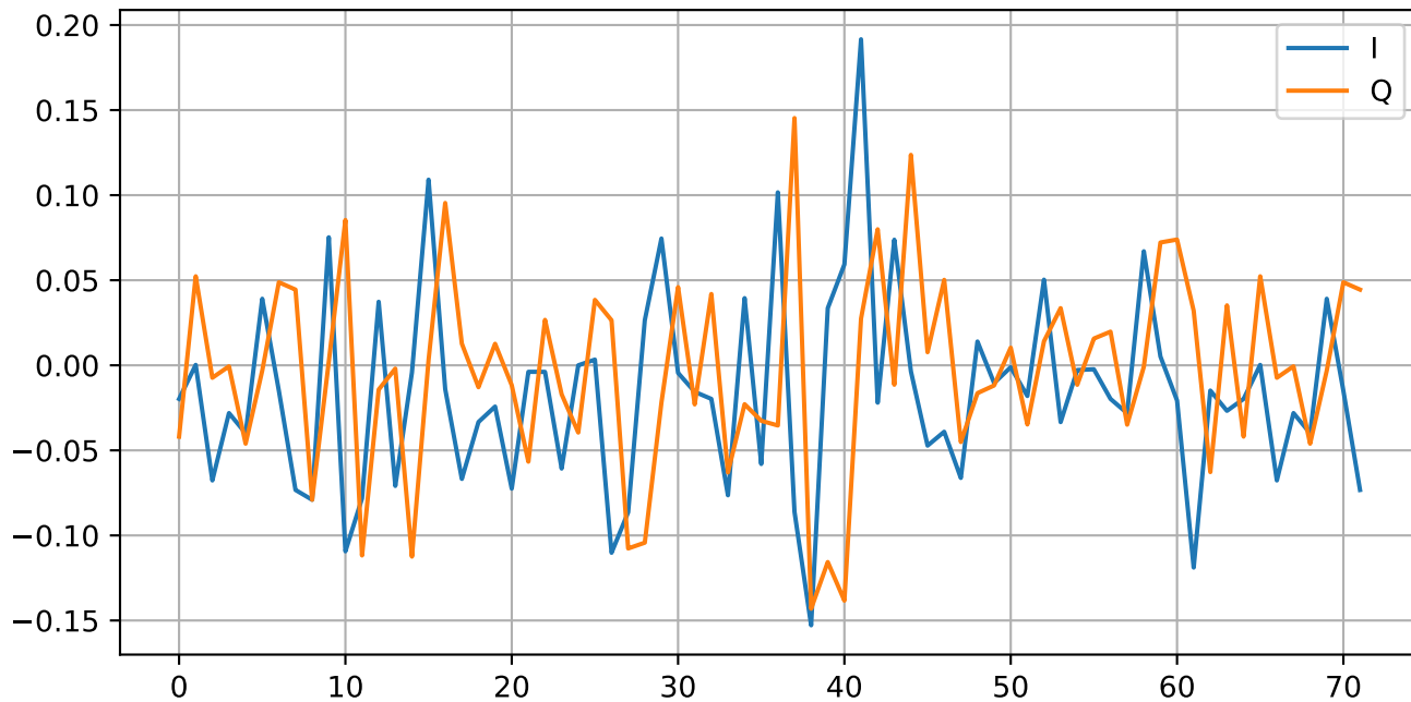
[UFONE] [CLEAN] OFDM (1)
