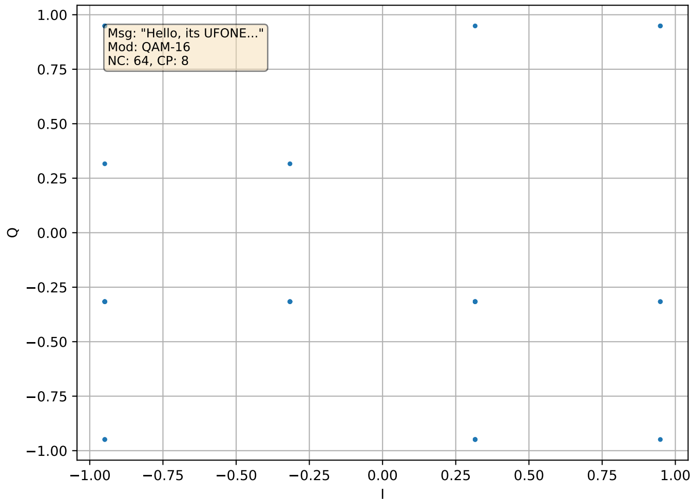
[MSG 0] R2 Constellation
