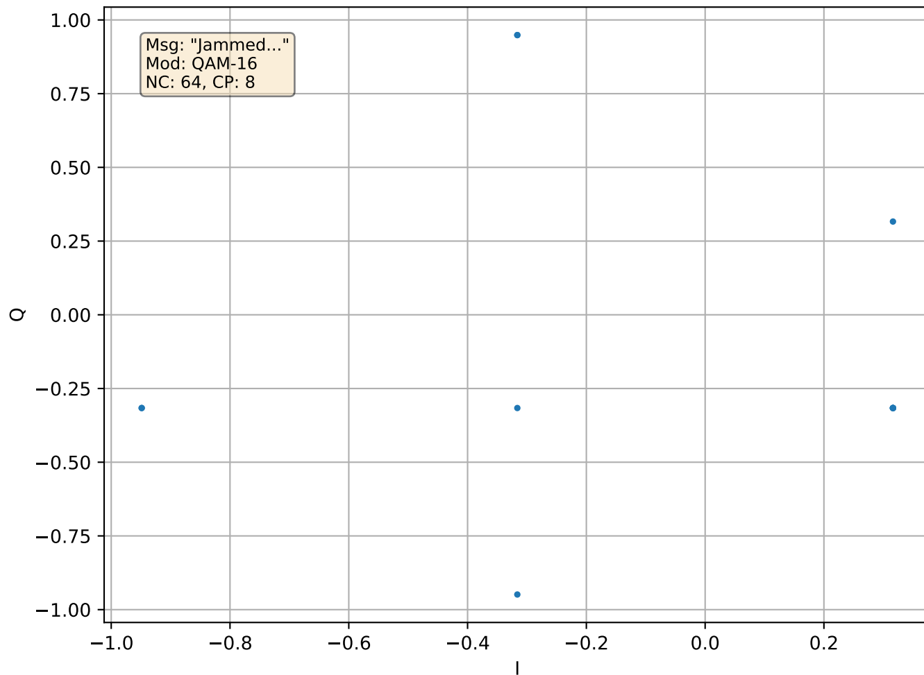
[MSG 10] R2 Constellation
