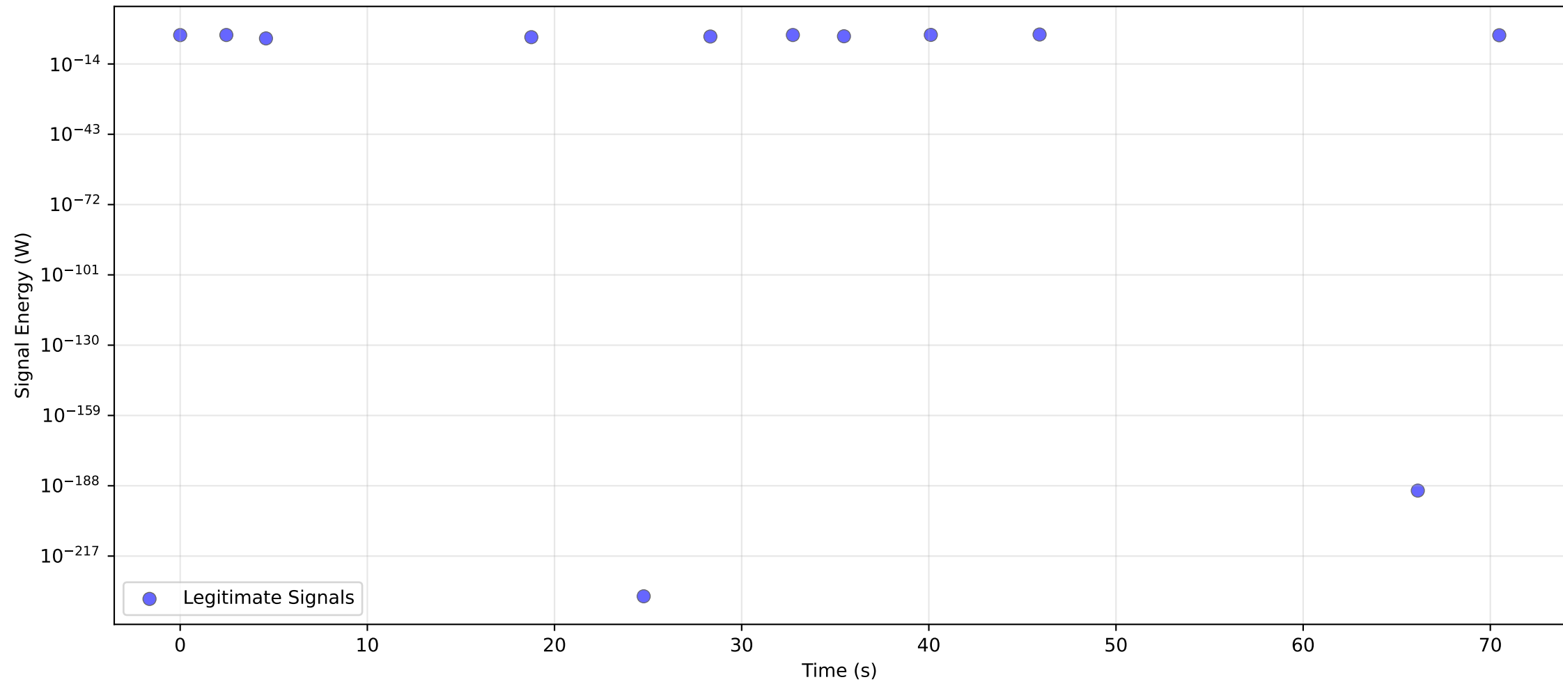
[BS BS1] Spectrum Sensing: Signal vs Jamming Overlay
