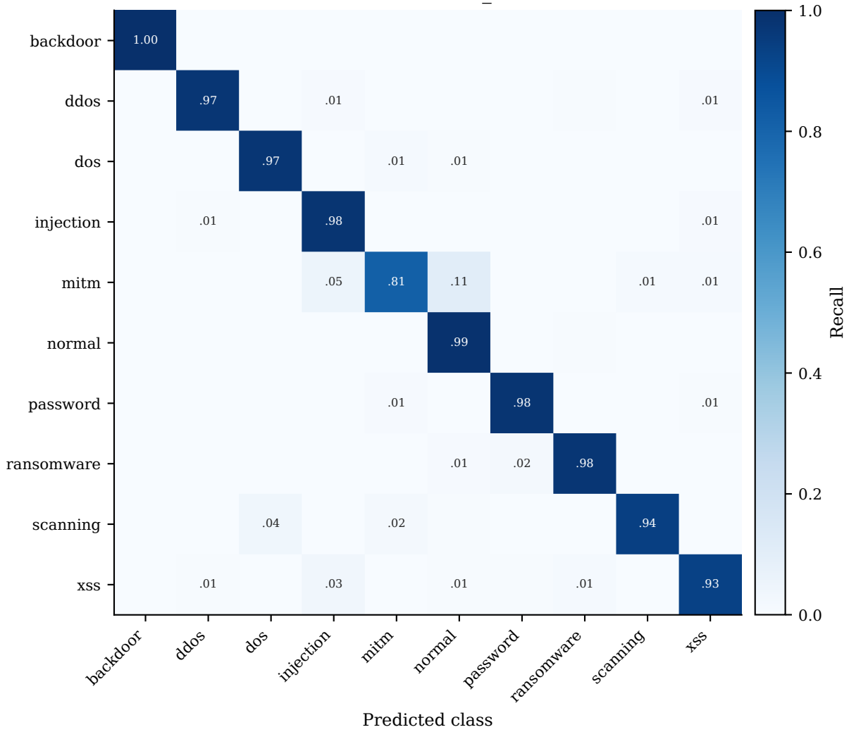
GB-META - ton_iot
