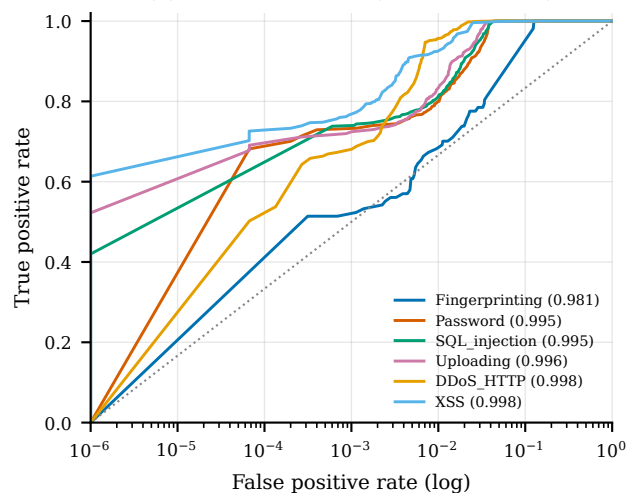
(b) ROC, one-vs-rest (worst 6 classes)
