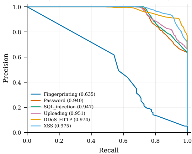
(c) Precision-recall (worst 6 classes)
