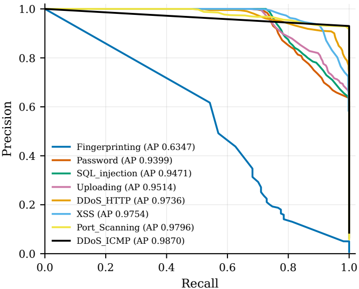
Precision-recall - edge_iiotset
