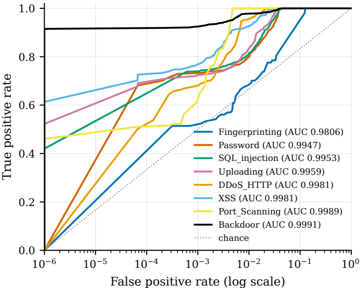
ROC (one-vs-rest) - edge_iiotset
