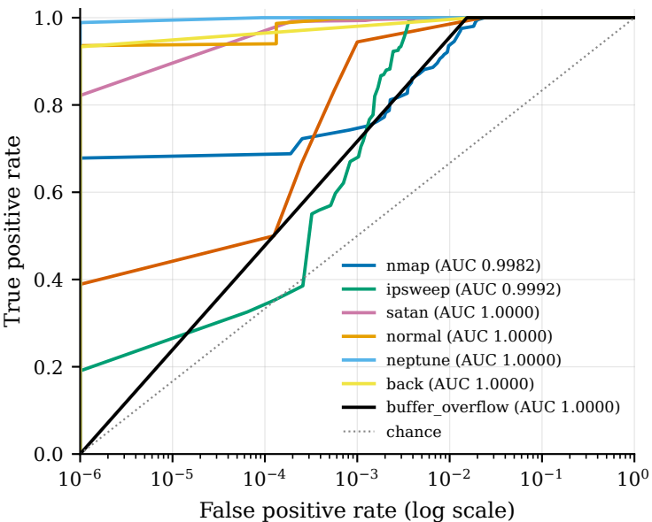
ROC (one-vs-rest) - nslkdd
