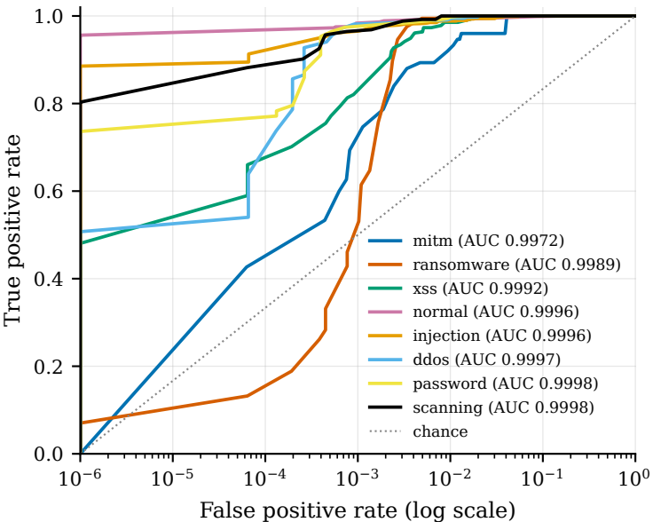
ROC (one-vs-rest) - ton_iot
