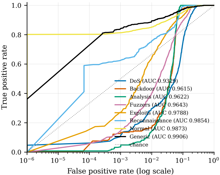
ROC (one-vs-rest) - unsw_nb15
