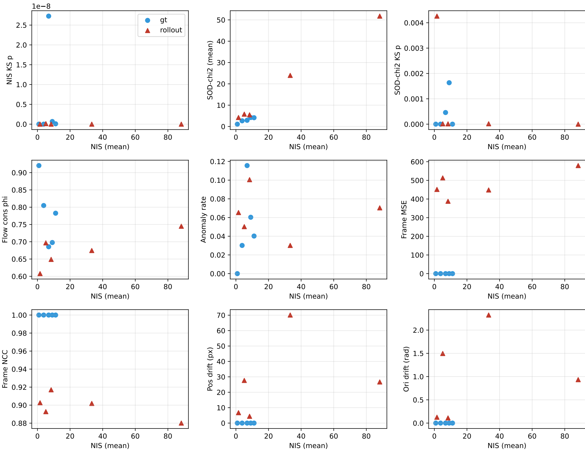
NIS (mean) vs other metrics, per episode
