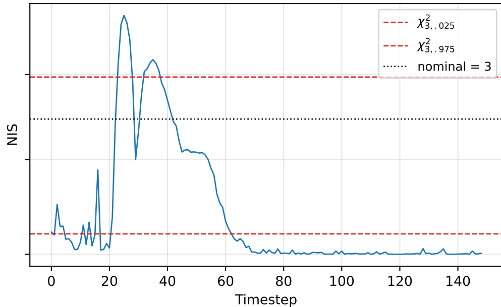
RI-EKF (sigma=10px, ep=0, real)
