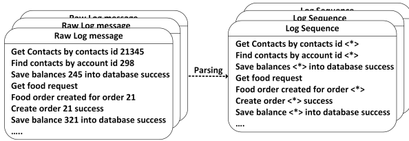
FIGURE 5. Employing the drain method for log parsing on raw log messages from the trainticket application.
