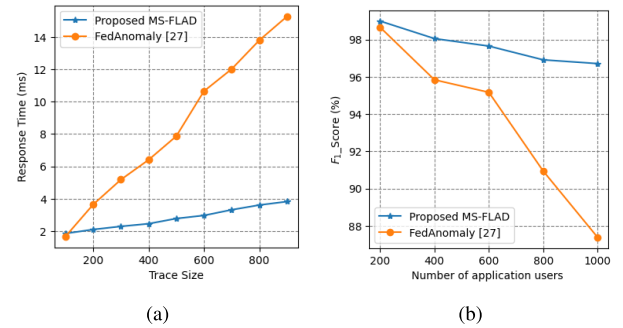
FIGURE 12. Scalability of the proposed MS-FLAD and FedAnomaly, in terms of (a) response time of prediction vs. trace size, (b) F_1 -score vs. the number of application users.
