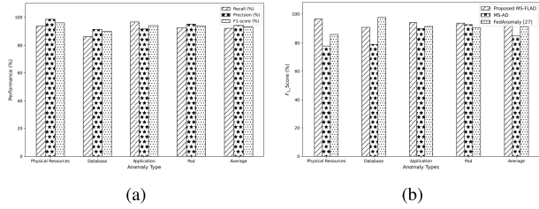
FIGURE 13. Performance evaluation: (a) Recall, precision, and F_1 -score of the proposed MS-FLAD across different anomaly types. (b) F_1 -score comparison across different anomaly types for MS-FLAD, MS-AD, and FedAnomaly [27].
