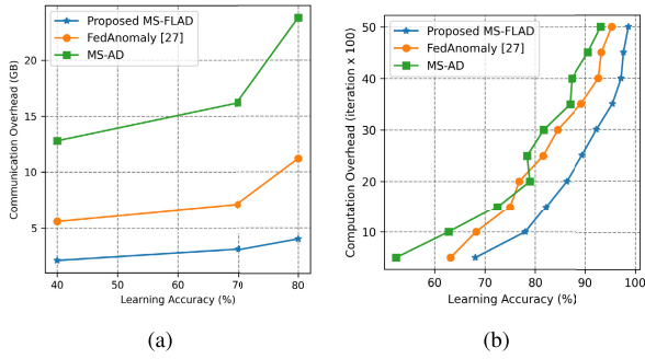
FIGURE 11. (a) Communication overhead vs. learning accuracy and (b) learning accuracy vs. computation overhead.
