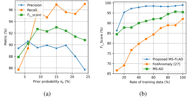
FIGURE 14. (a) Impact of prior probability, \pi_p , on the proposed MS-FLAD performance, (b) F_1 -score vs. different training data rate.
