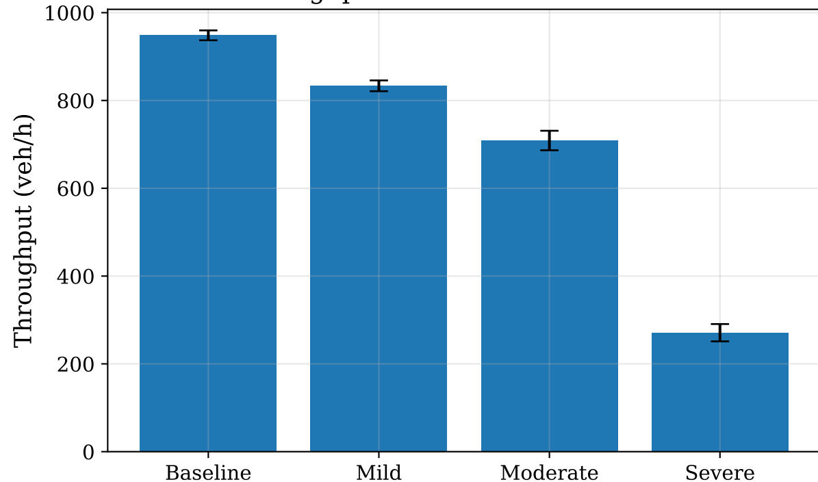
Throughput Across Flood Scenarios
