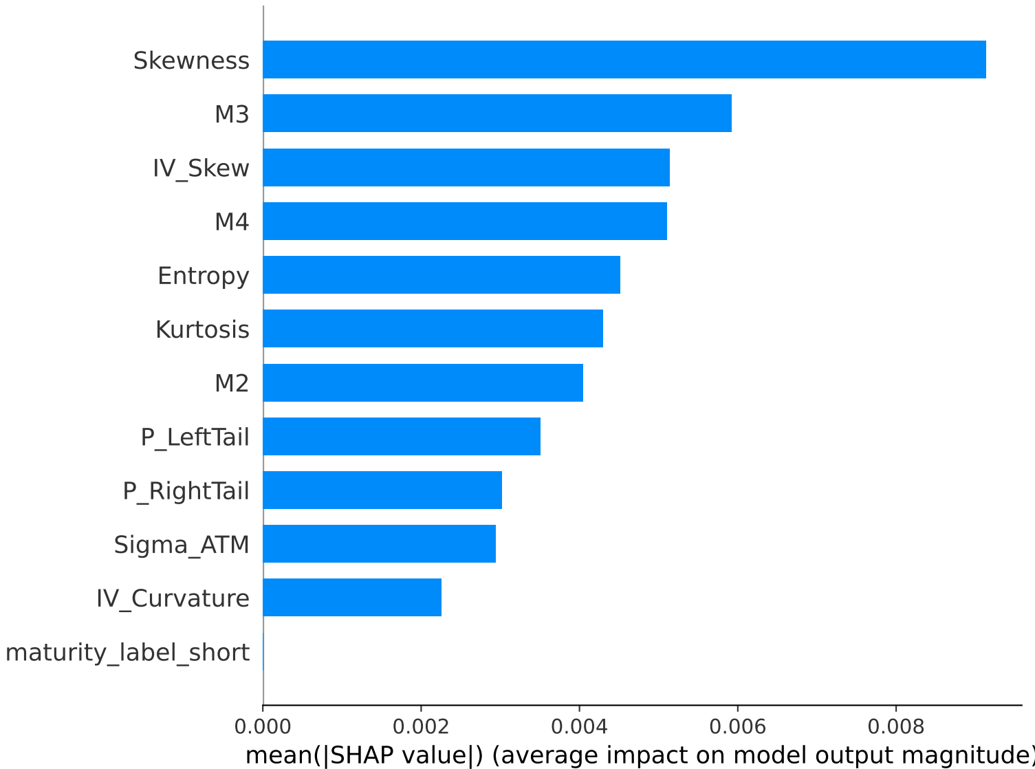
Feature Importance (Random Forest - Mean)
