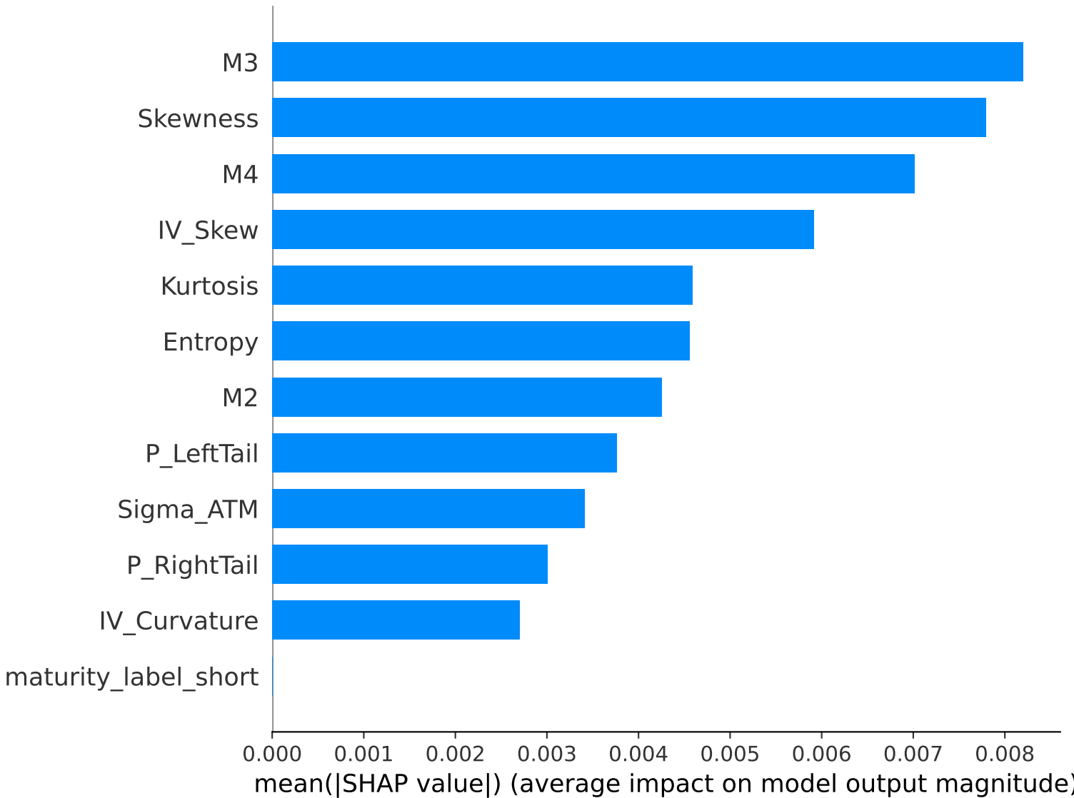
Feature Importance (Random Forest - Median)
