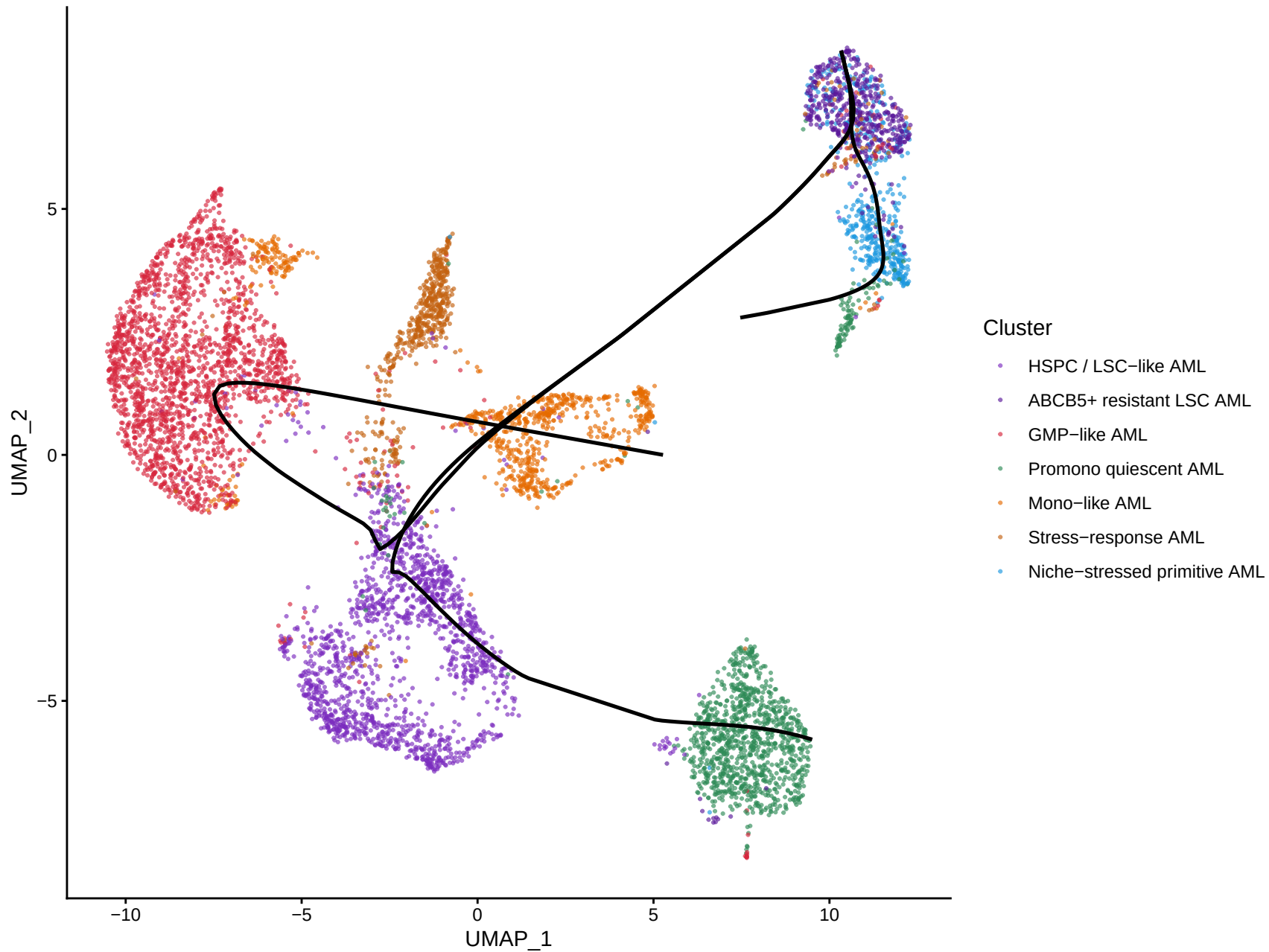
AML lineages – Slingshot (root: ABCB5+ resistant LSC AML)
