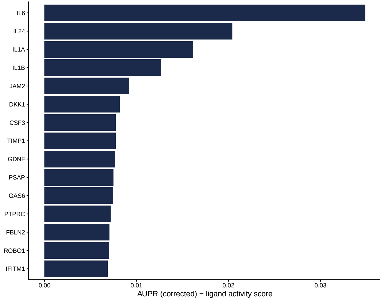
NicheNet ligand activity -> Promono quiescent AML
