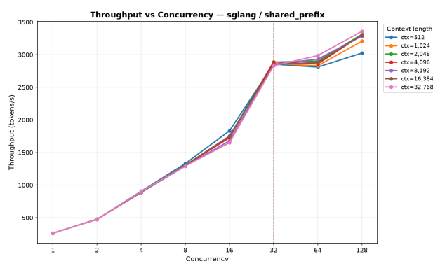
Figure 6.2: SGLANG TP=2 throughput — shared_prefix
