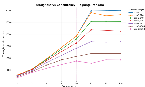
Figure 6.1: SGLANG TP=2 throughput — random
