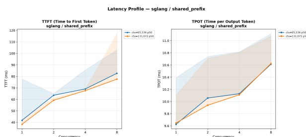
Figure 5.4: Long-ctx latency — shared_prefix
