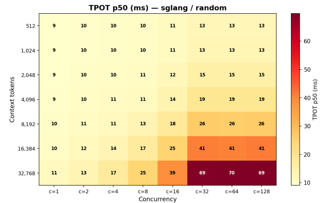
Figure 1.4: TPOT p50 heatmap (ctx × concurrency)
