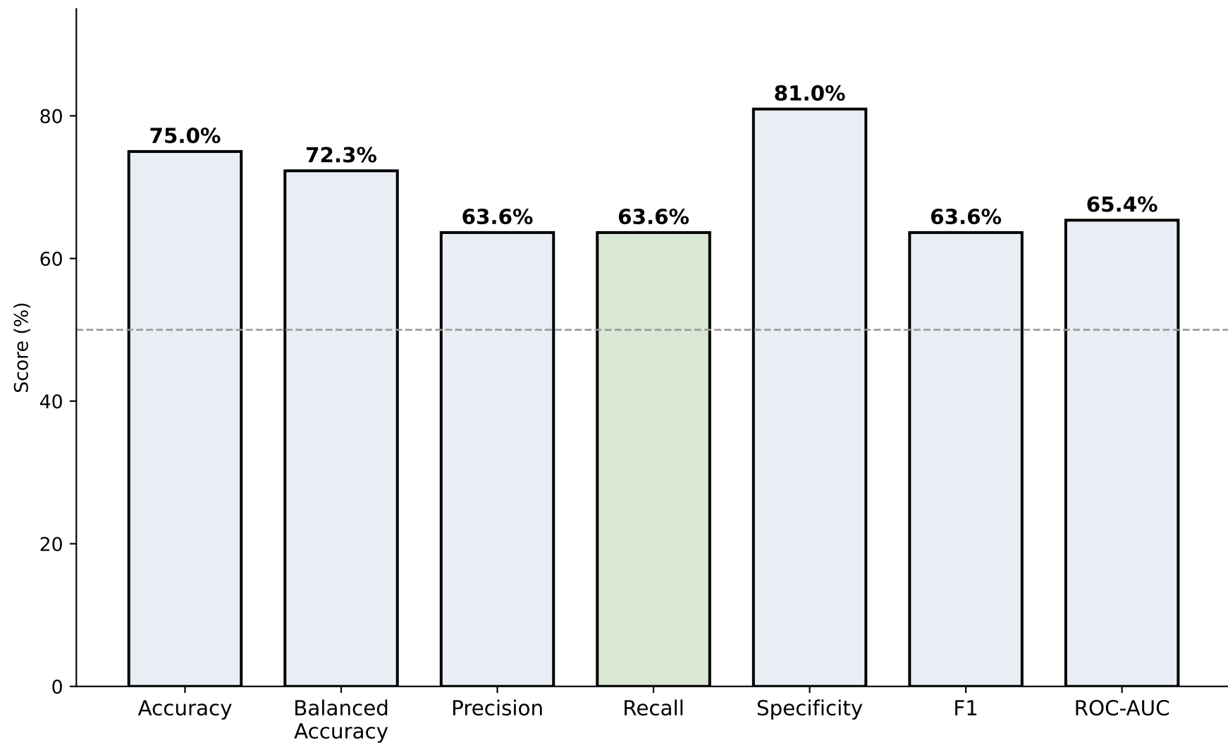
Figure 7.2 Held-out Classification Metrics (Deployed Random Forest)
