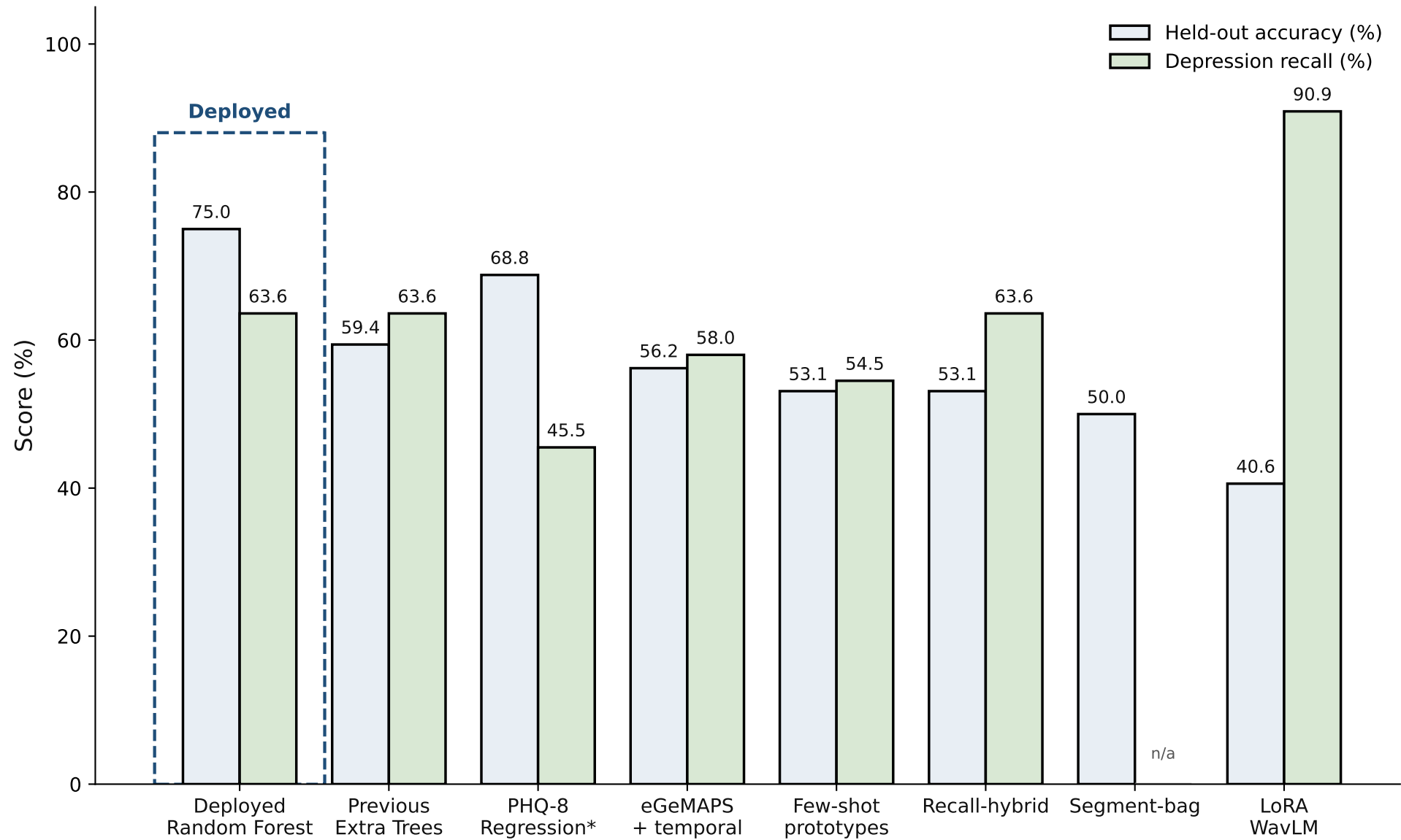
Figure 7.3 Experimental Candidate Comparison (Held-out)
