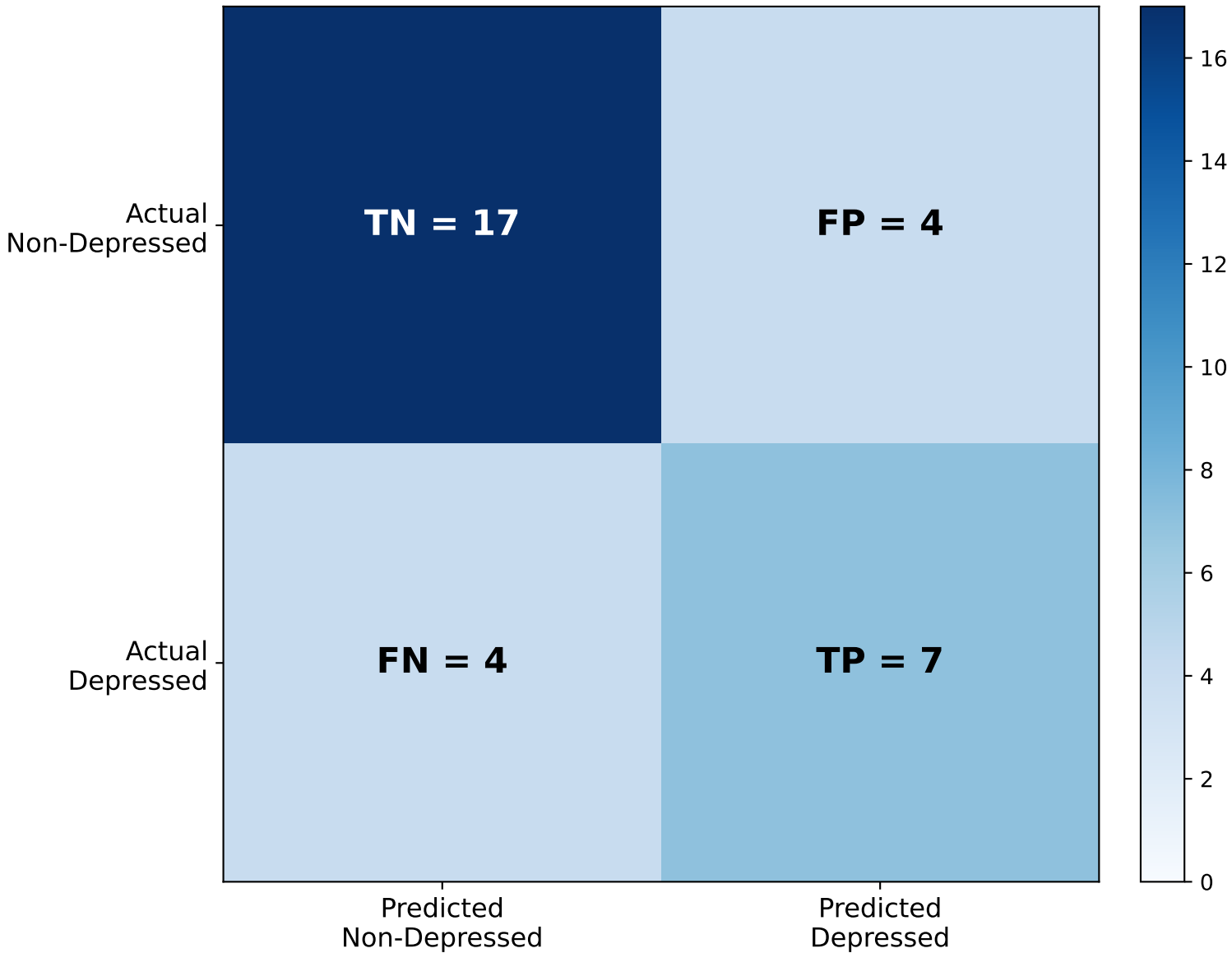
Figure 7.1 Confusion Matrix — Held-out Test (n = 32)
