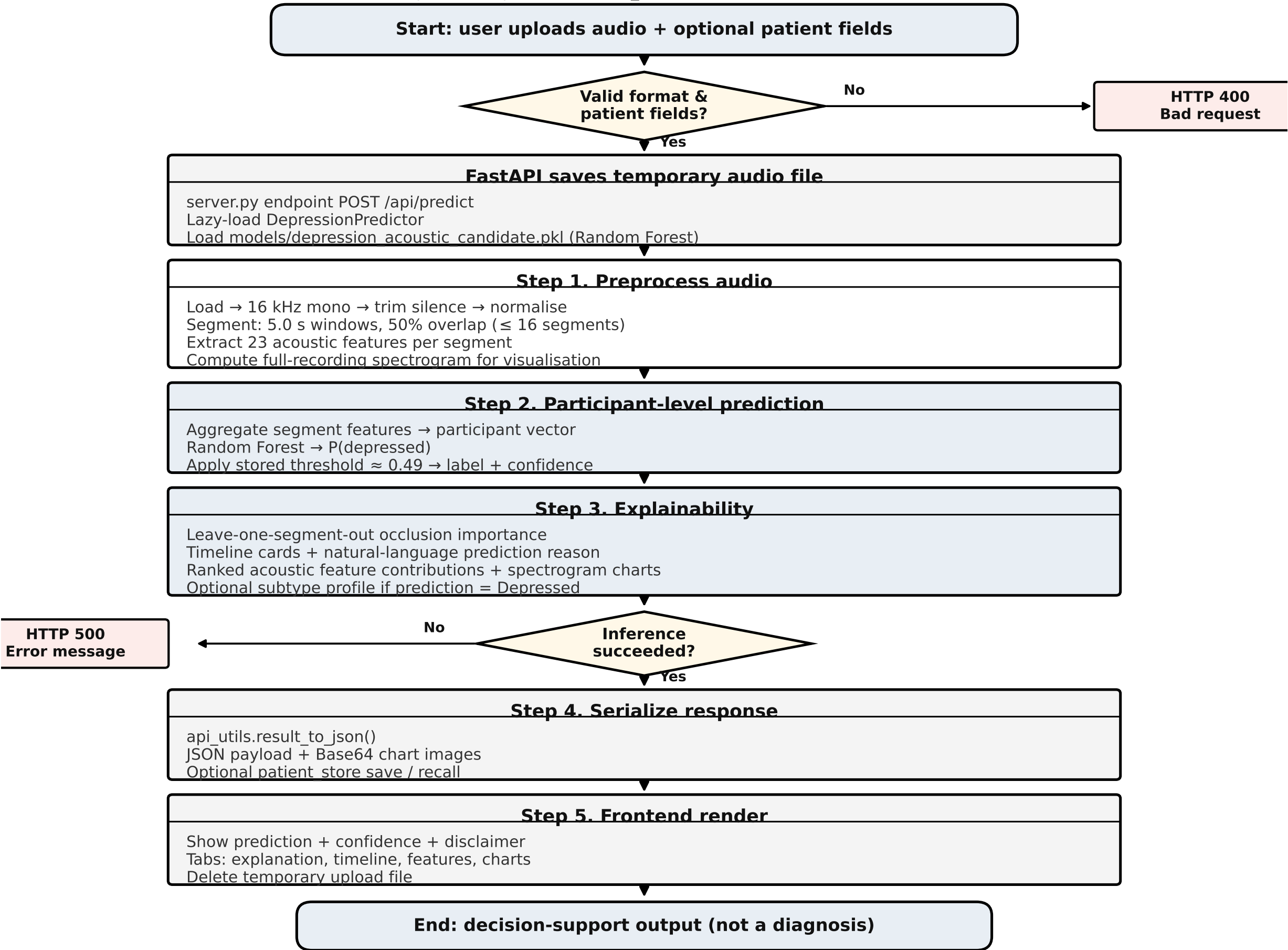
Figure 6.2 InferencePipeline Flowchart
