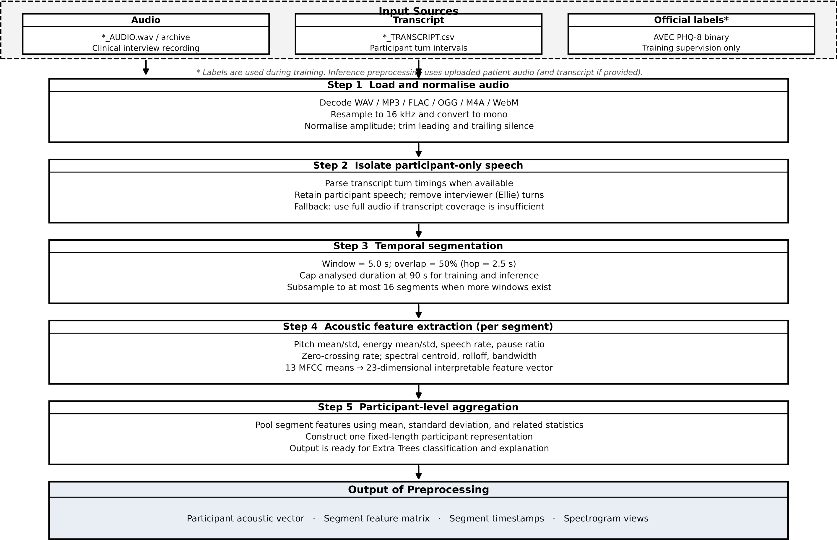
Figure 4.2 Preprocessing Pipeline
