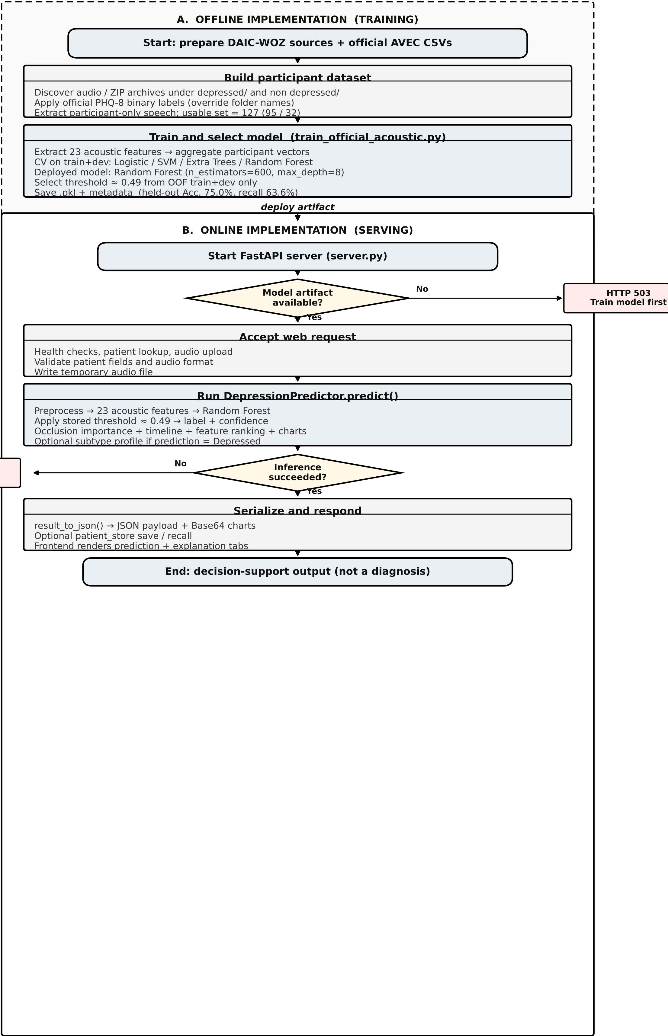
Figure 6.1 System Implementation Flowchart
