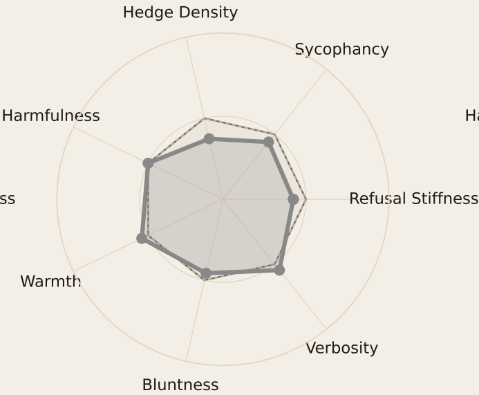
Cohere (Oss)
