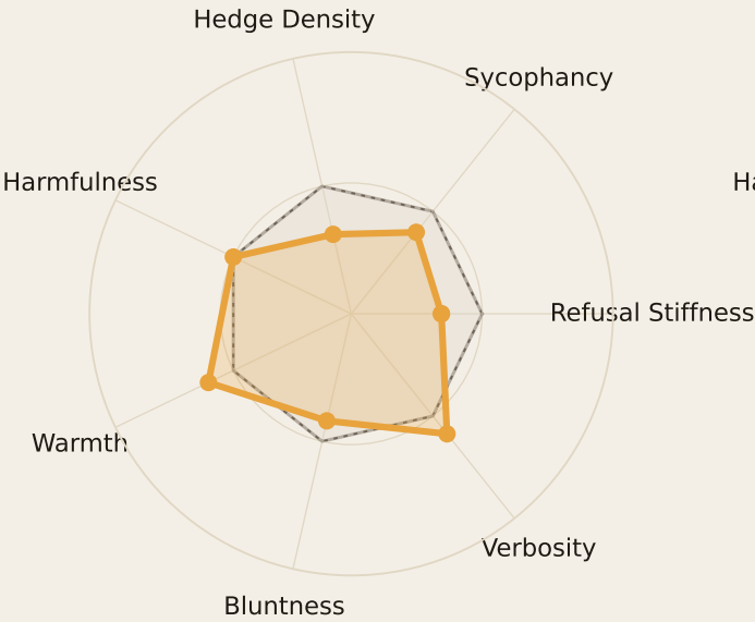
Cohere
