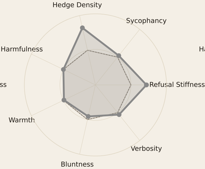
Mistral
