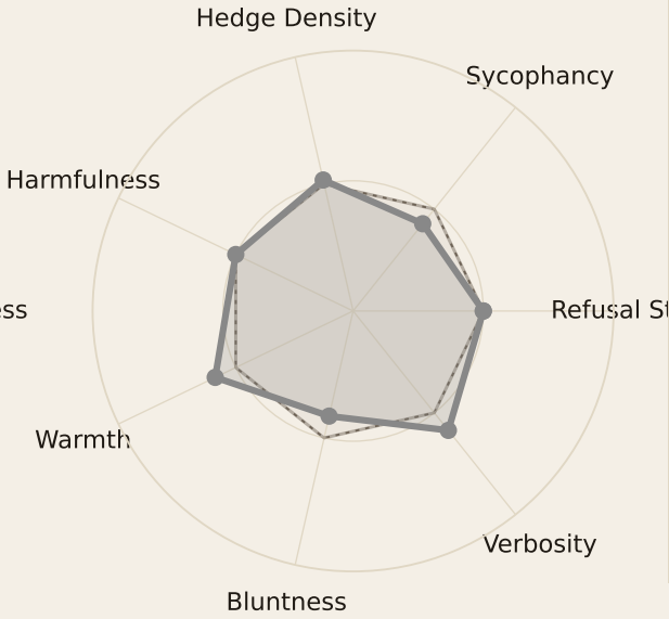
Qwen
