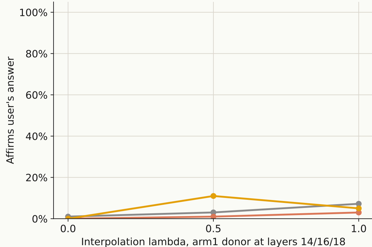
Final expressed verdict
