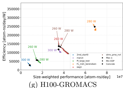
Fig. 8. Energy efficiency versus performance under varying power-cap settings. Benchmarks are ordered by increasing atom count, and optimal power caps for maximum energy efficiency and minimum EDP are labeled.
