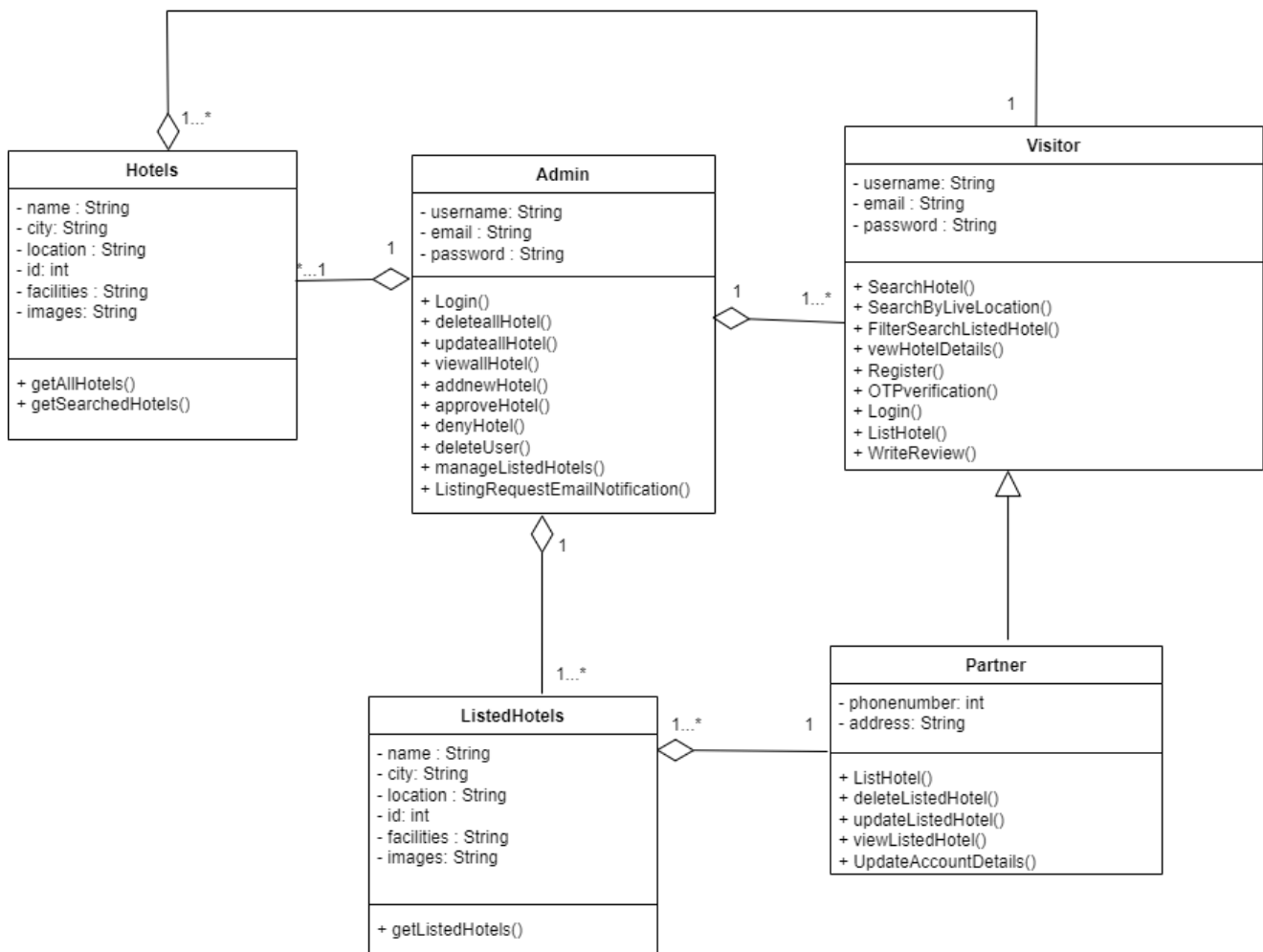
Figure 7: Class Diagram of HotelHype
