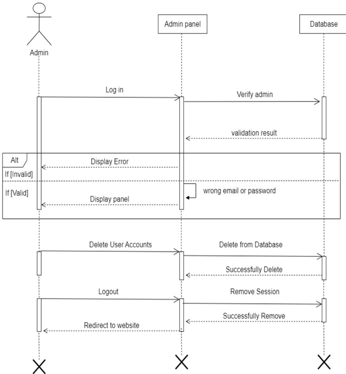
Figure 11: Sequence Diagram of Admin Login
