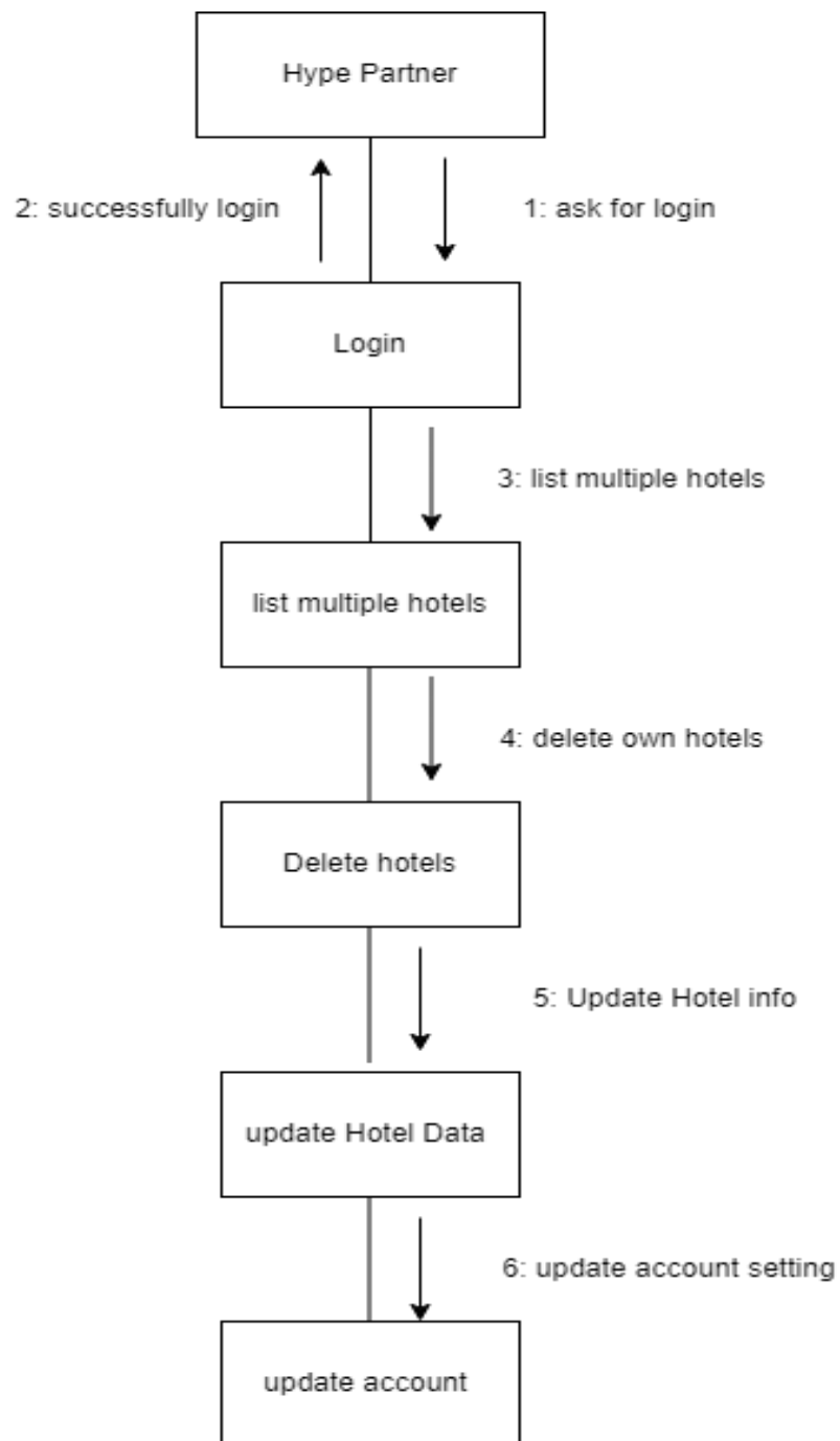
Figure 9: Collaboration Diagram of Partner
