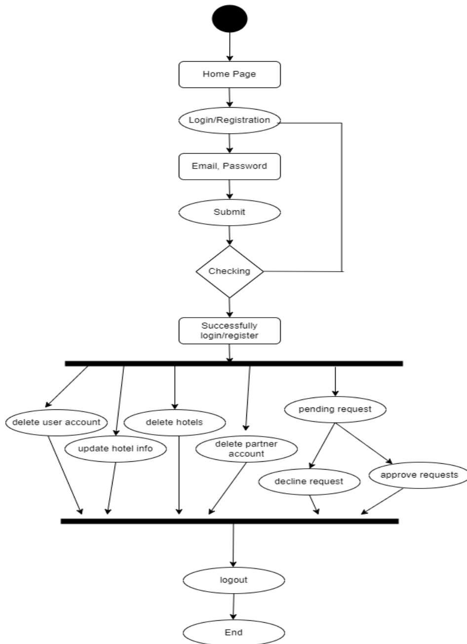
Figure 17: Activity Diagram of Admin
