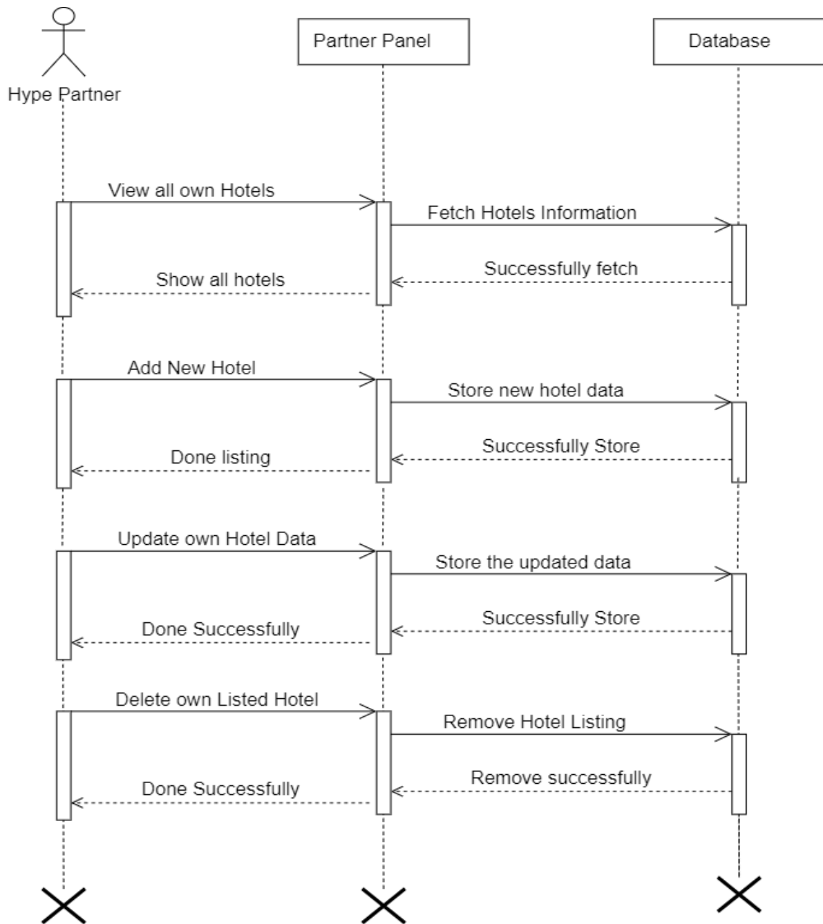
Figure 14: Sequence Diagram of Partner Listed Hotel Management
