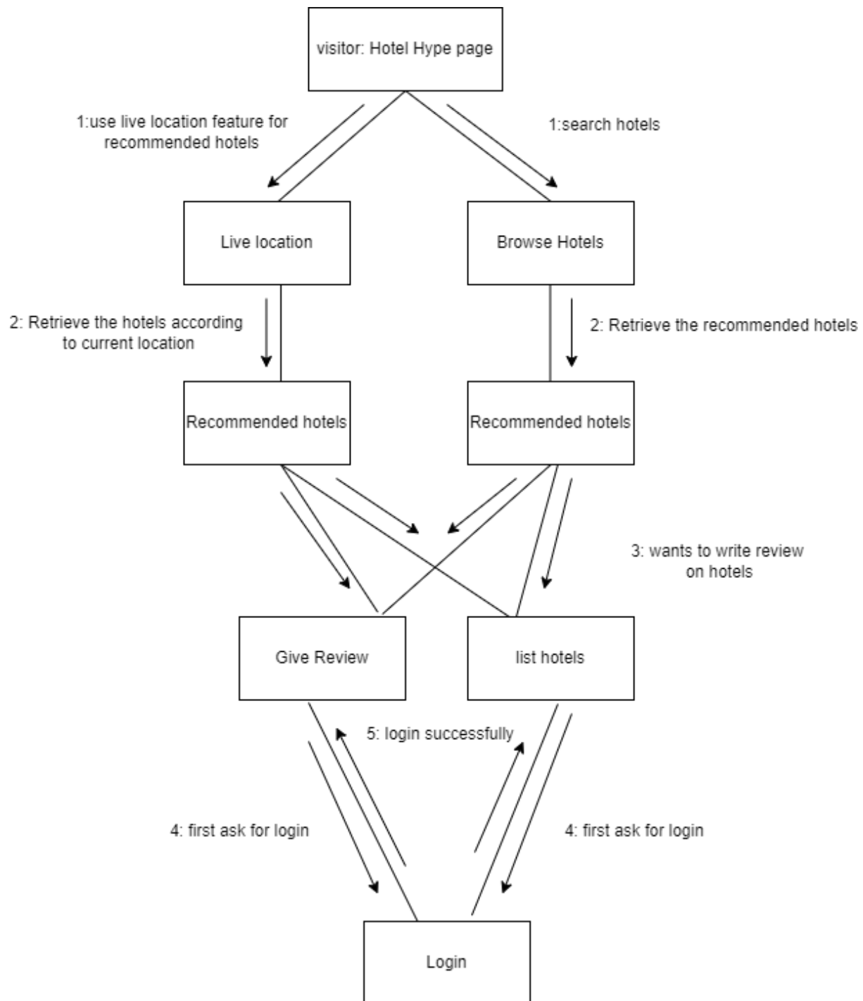
Figure 10: Collaboration Diagram of Visitor
