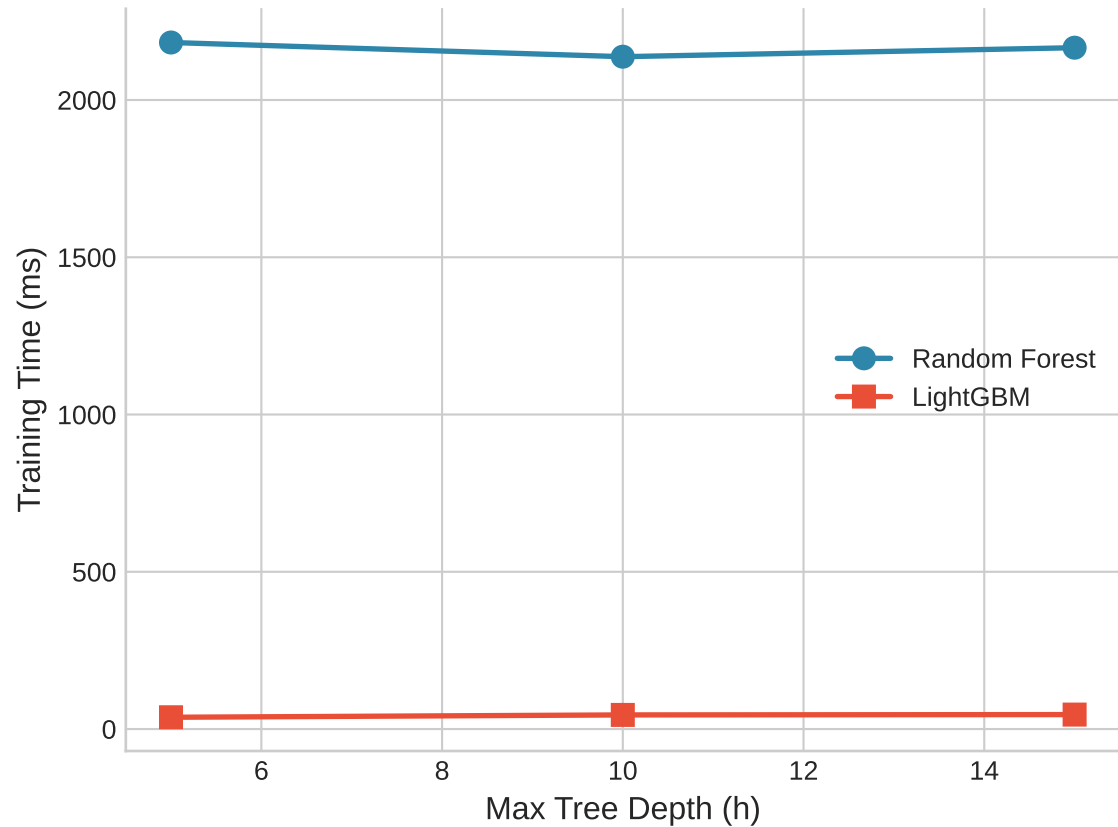
Training Time vs Tree Depth (n_estimators=100)
