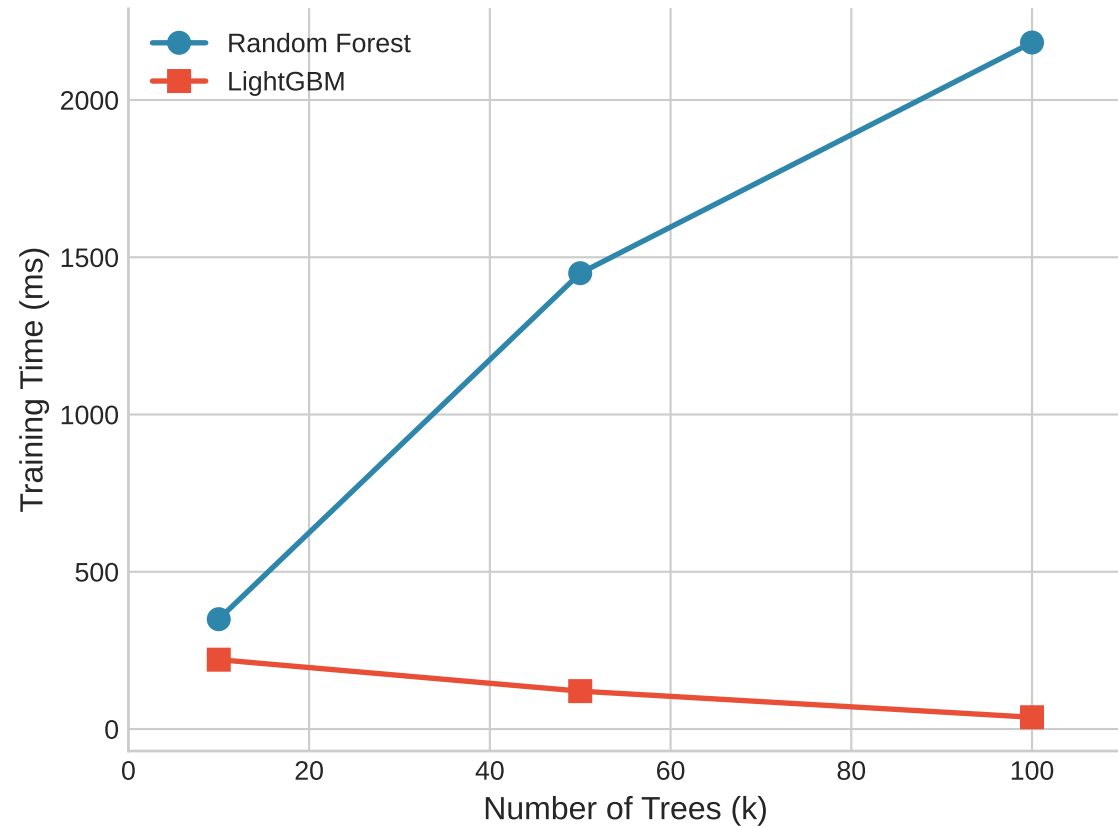
Training Time vs Ensemble Size (max_depth=5)
