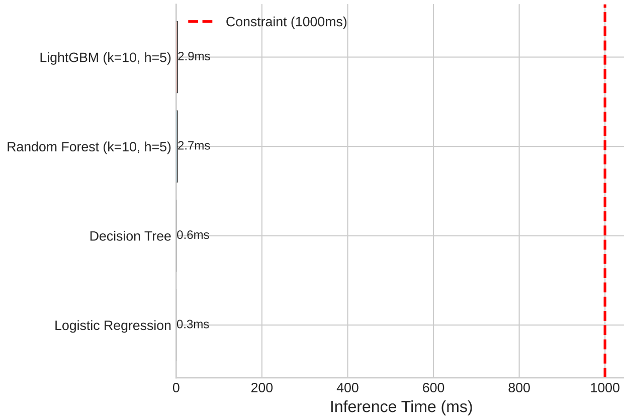
Inference Latency Comparison
