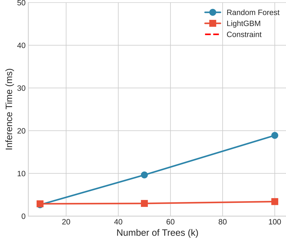
Inference Time Scaling (26 test samples)
