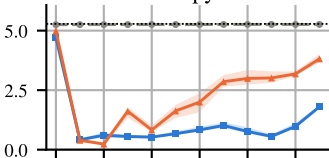
Attention entropy
