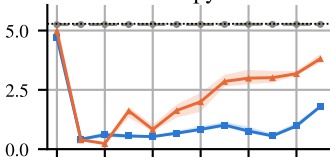
Attention entropy
