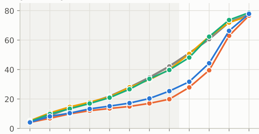
probe, epoch 299
