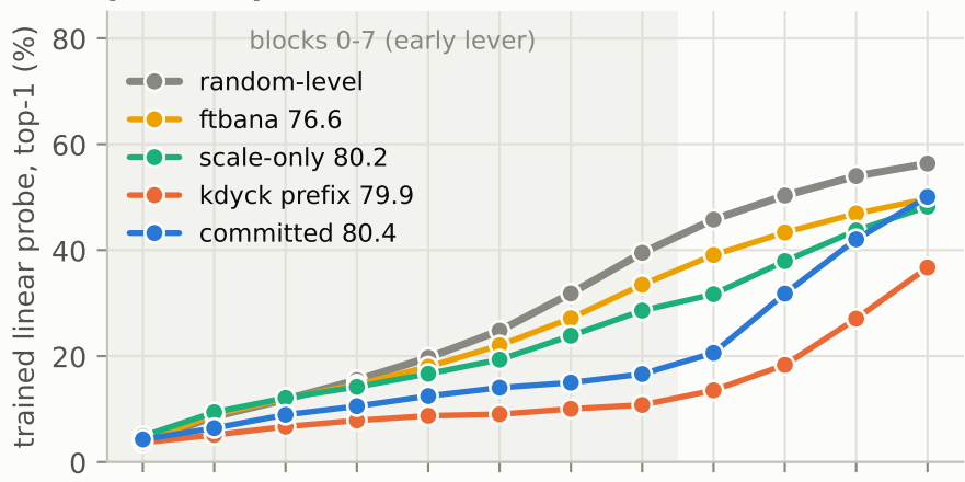
probe, epoch 29
