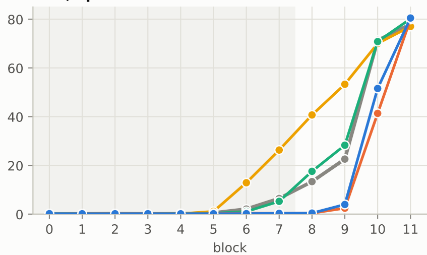
lens, epoch 299
