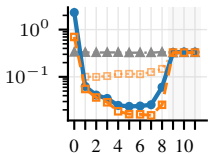
GELU output rms
