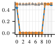
active fc1 units
