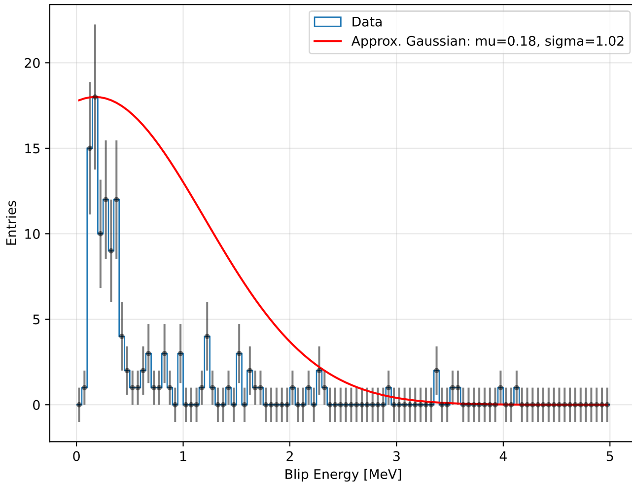
Blip Energy Distribution with Approx. Gaussian
