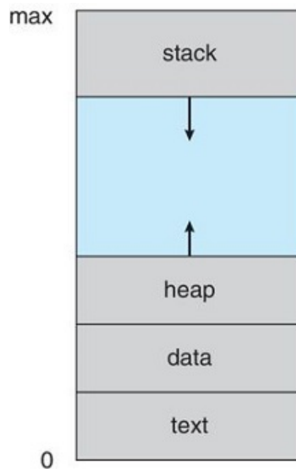
Figure 2.1.1: Layout of a process in memory.
