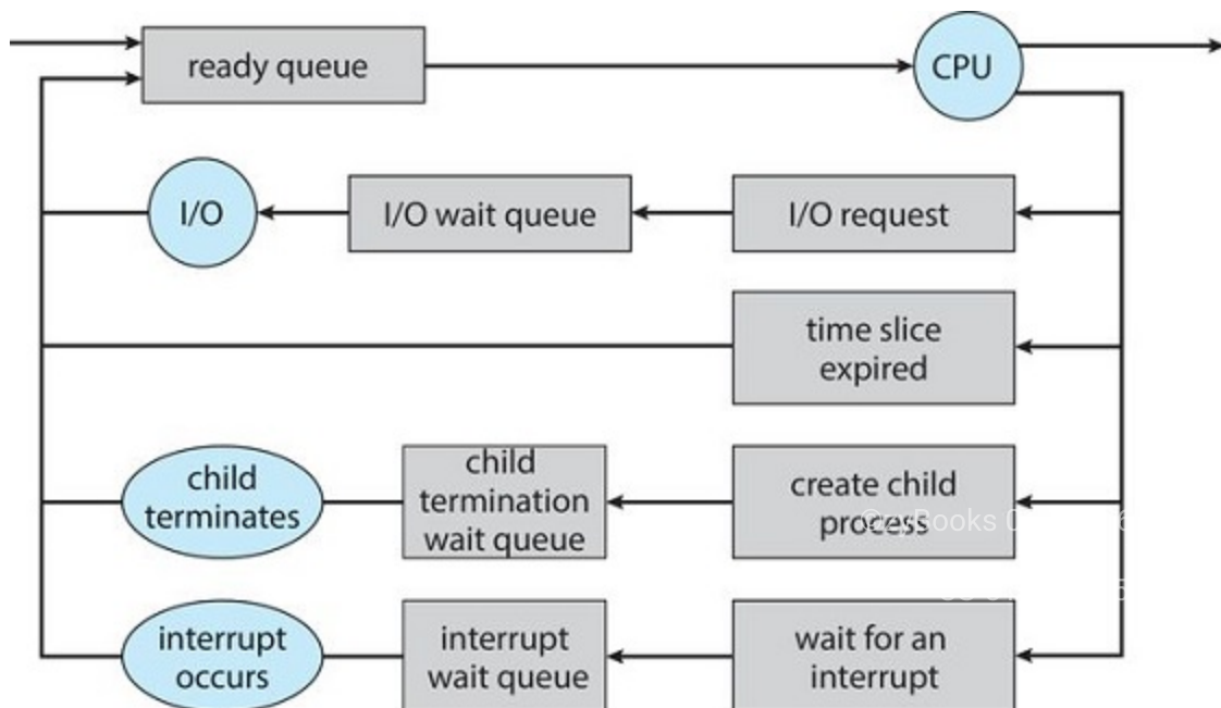
Figure 2.2.2: Queueing-diagram representation of process scheduling.
