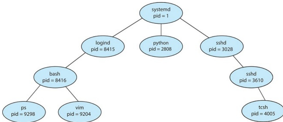
Figure 2.3.1: A tree of processes on a typical Linux system.
