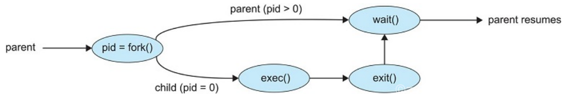
Figure 2.3.3: Process creation using the fork() system call.
