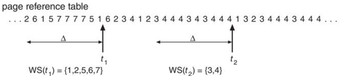
Figure 7.6.3: Working-set model.
