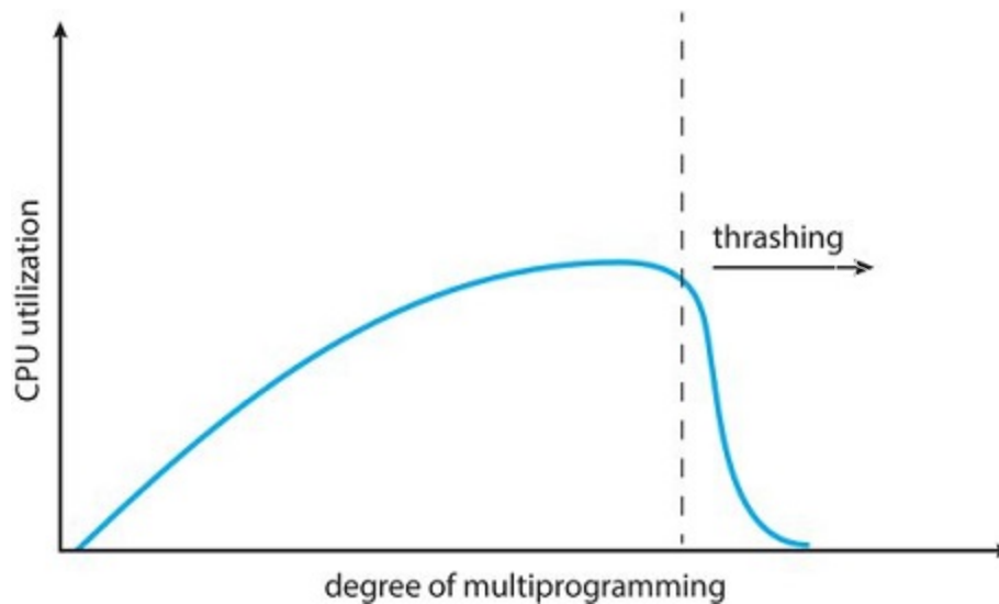
Figure 7.6.1: Thrashing.
