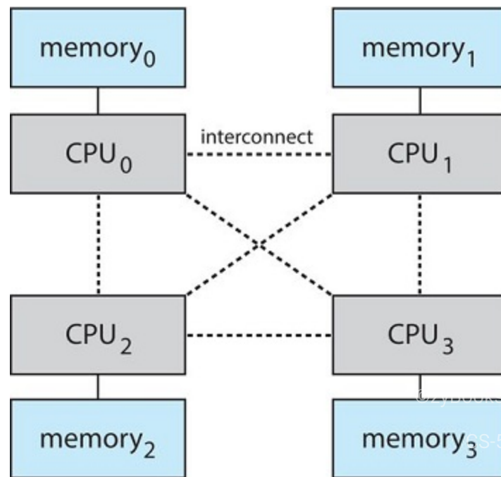
Figure 7.5.2: NUMA multiprocessing architecture.
