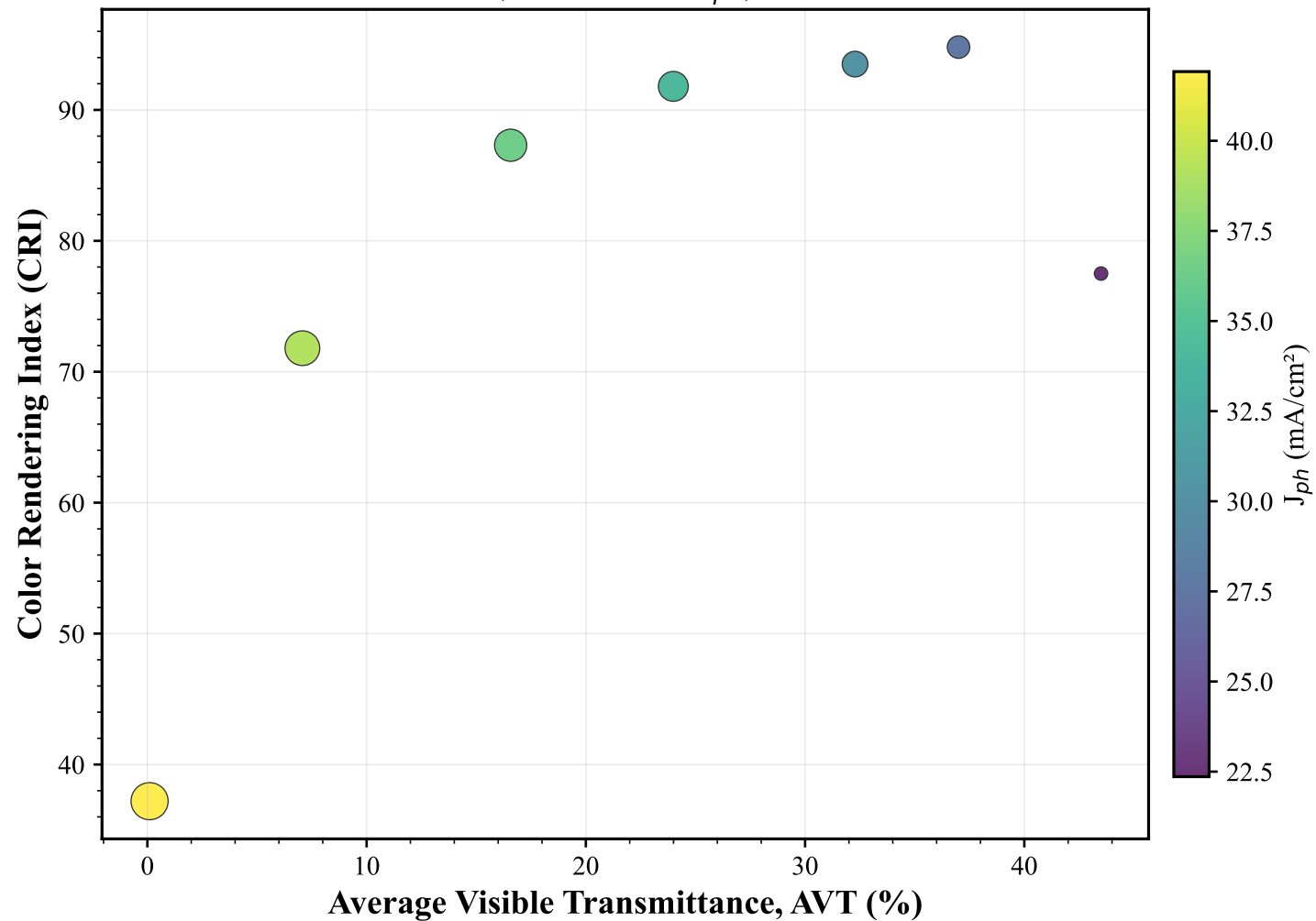
Pareto Designs: AVT vs CRI (Bubble size \propto J_{ph} )
