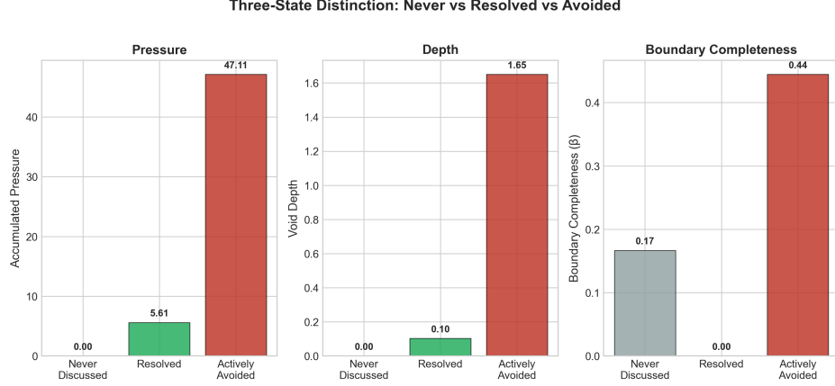
Figure 3: Three-state behavioral signatures. Each state has a unique profile; Bayesian baselines cannot distinguish S1 from S3.
