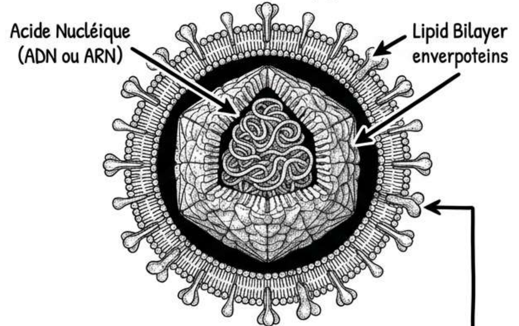
Virus Enveloppé
