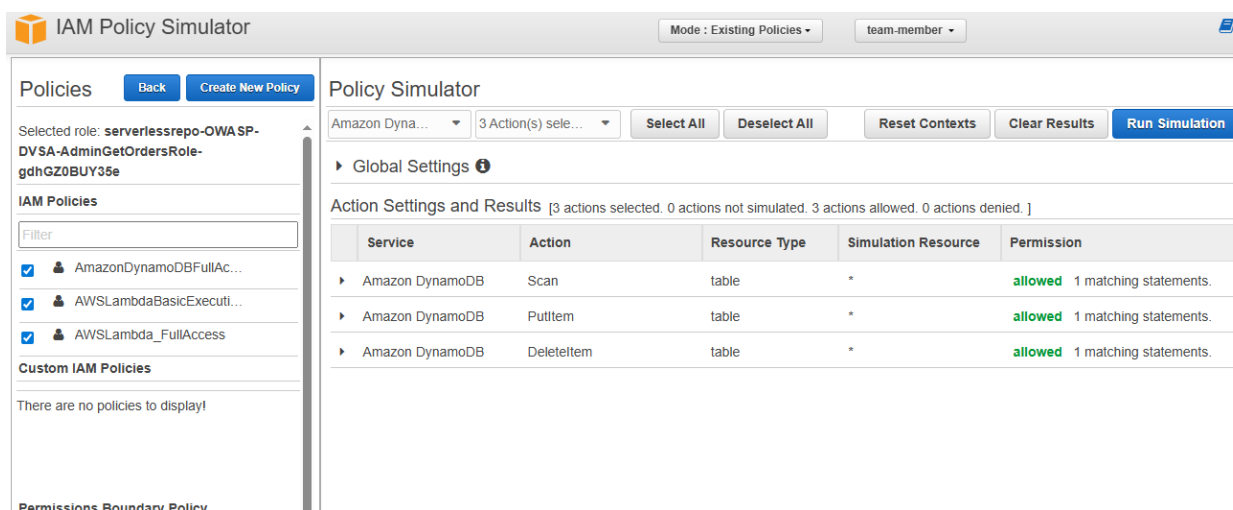
Figure 4: IAM Policy Simulator showing that the Lambda execution role allows DynamoDB actions such as Scan, PutItem, and DeleteItem (result: Allowed).
